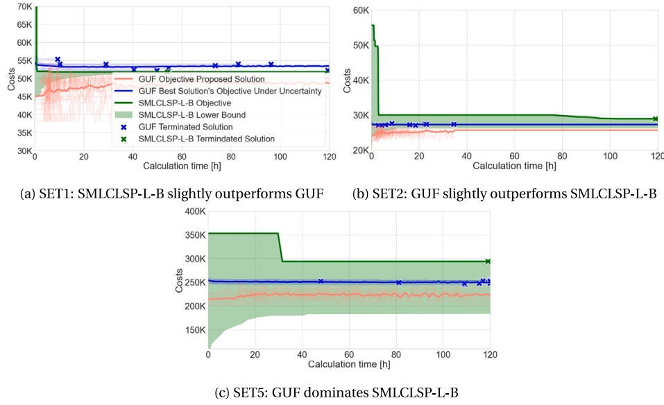
Fig. 7. Time-dependent model performance on D2T2 for three representative cases.
