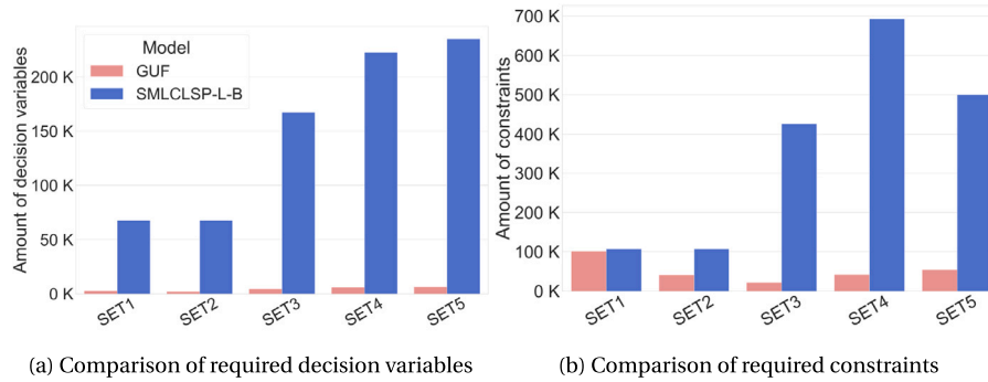
Fig. 5. Model complexity analysis.
