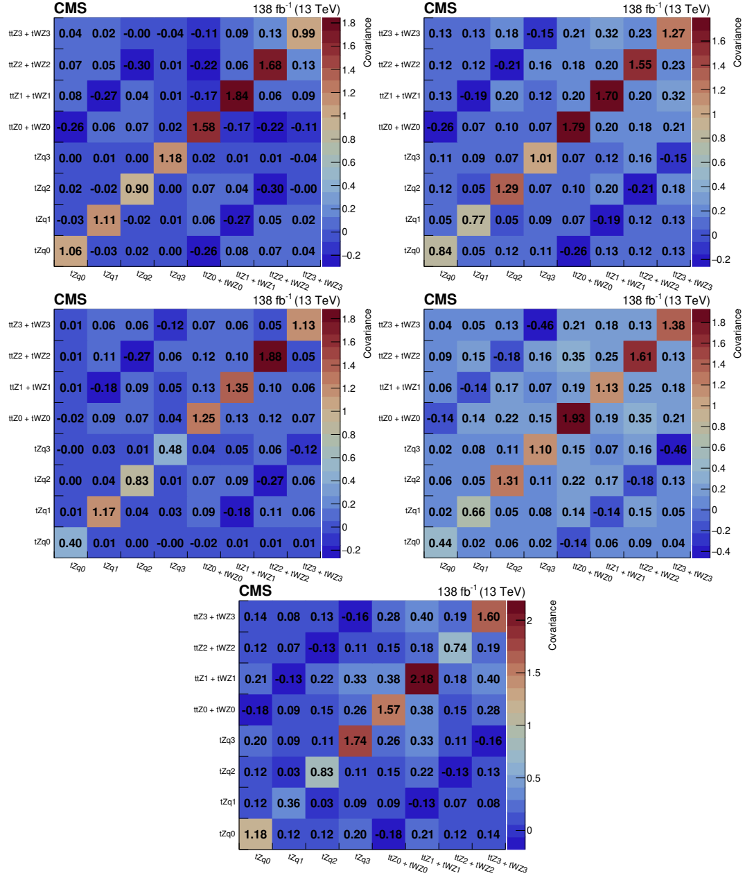
Figure 15. Covariance matrices for the simultaneous measurement of the differential cross section as a function of p_T(Z) , p_T(\ell_W) (upper right), \Delta R(Z, \ell_W) (middle left), \Delta\phi(\ell^+, \ell^-) (middle right), and \cos\theta_Z^* (lower). The last digits in the axis labels refer to the respective bin of the corresponding differential cross section measurement.
