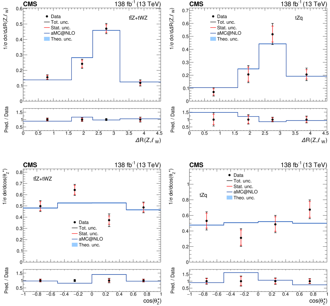
Figure 14. Normalized differential cross sections for the sum of t\bar{t}Z and tWZ production (left column) and tZq production (right column) as a function of \Delta R(Z, \ell_W) (upper), and \cos\theta_Z^* (lower). The inner (outer) error bars indicate the statistical (total) uncertainty, while the shaded area refers to the uncertainty in the theory prediction. The lower panel shows the ratio of the prediction with the data. The points at unity show the uncertainty of the data.
