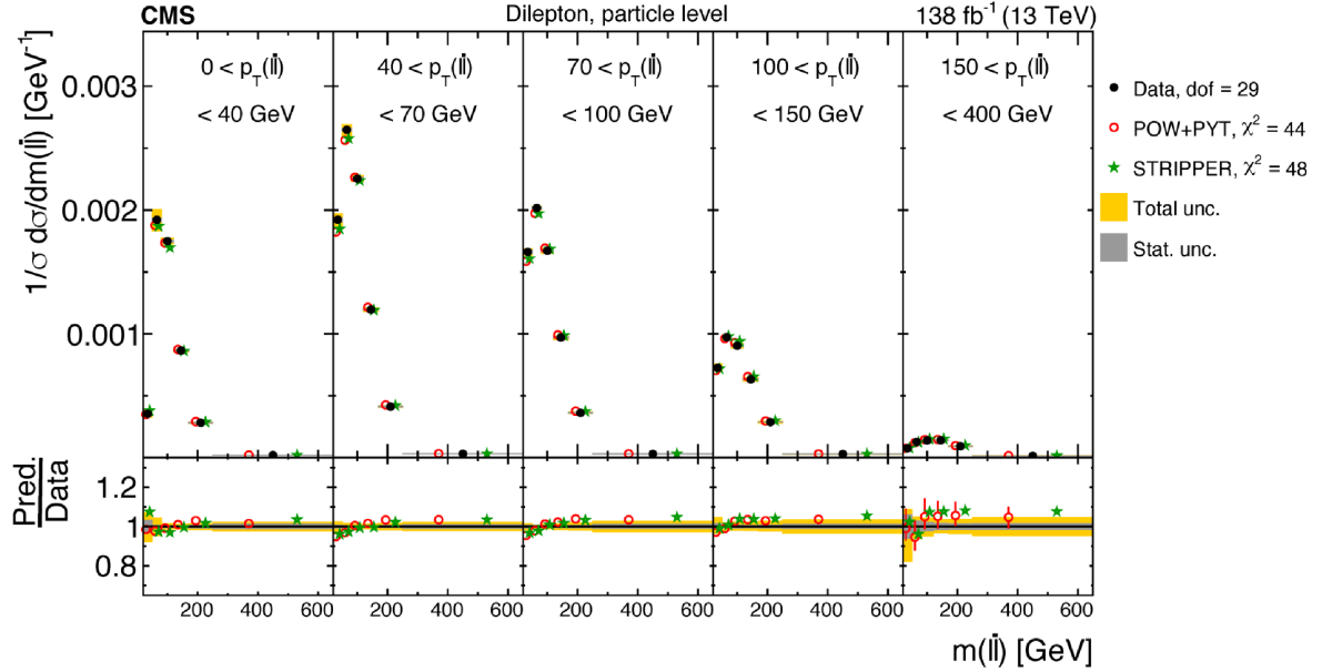
Figure 63. Normalized [p_T(\ell\bar{\ell}), m(\ell\bar{\ell})] cross sections are shown for data (filled circles), POWHEG+PYTHIA 8 (‘POW-PYT’, open circles) simulation, and STRIPPER NNLO calculation (stars). Further details can be found in the caption of figure 57.
