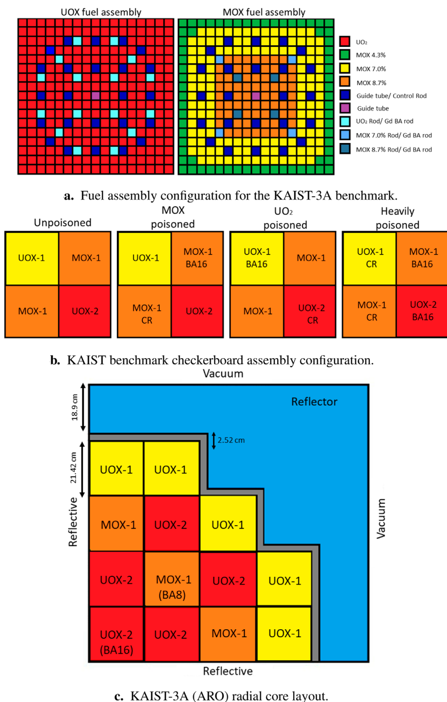
FIGURE 2 KAIST-3A benchmark geometry. (A) Fuel assembly configuration for the KAIST-3A benchmark. (B) KAIST benchmark checkerboard assembly configuration. (C) KAIST-3A (ARO) radial core layout.
