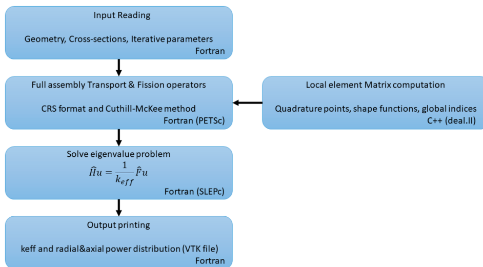
FIGURE 1 KANECS calculation scheme.
