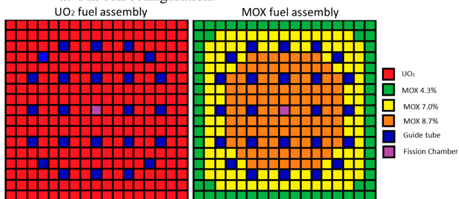
b. Fuel assembly configuration for the C5G7 benchmark.
