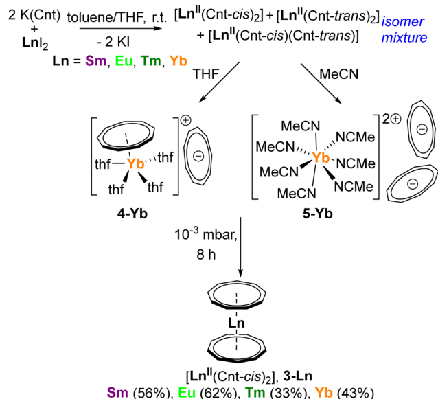
Scheme 4 Synthesis of the homoleptic Ln bis(Cnt) complexes as isomer mixture and the further isomerisation to the [Ln II (Cnt-cis) 2 ] complexes 3-Ln.
