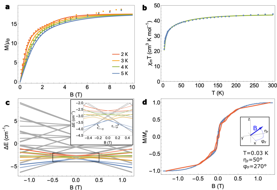
Fig. 4 | Experimental and theoretical simulations of \text{CrDy}_3 magnetic properties. a Comparison of the experimental isothermal powder magnetisation (dots) with the simulated powder magnetisation (solid lines) at T = 2, 3, 4 and 5 K. b Comparison of the experimental zero-field powder magnetic susceptibility versus temperature (blue dots) with the simulated \chi_m T (green solid line). c Zeeman energy levels of the thirty-two dimensional Hilbert space of \text{CrDy}_3 using J_1 = -0.4 \text{ cm}^{-1} and J_2 = -0.01 \text{ cm}^{-1} obtained from fitting to (a, b). The coloured lines correspond to Zeeman energies of states with a vortex configuration of the \text{Dy}^{\text{III}} magnetic moments (the lighter (darker) colour represents a clockwise (anticlockwise) vortex configuration). The applied field is chosen almost exactly along the intrinsic magnetic
