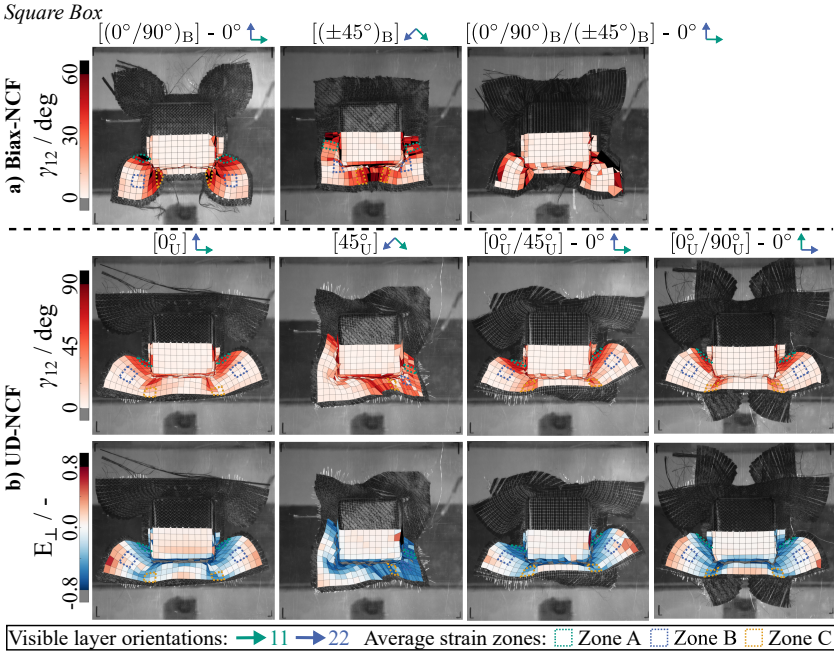
Figure 4.41: Relevant DIC-strains in the square box shape forming test with different layup orientations at a maximum tool displacement of 85 mm [207].
