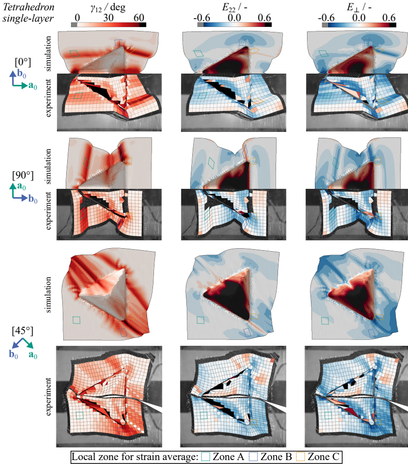
Figure 5.20: Comparison of experimental and simulative strains for [0°], [45°] and [90°] single-layer setups in the tetrahedron forming tests for a punch displacement of u = 95 mm [294].
