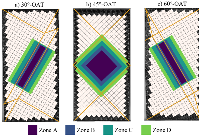
Figure A.12: Overview of different areas with increasing size for an averaging of the strain components | 30°- and 60°-OAT: Smallest zone with 130 mm \times 10 mm (A) whose width is increased symmetrically in increments of 20 mm | 45°-OAT: Smallest zone with 60 mm \times 60 mm (A) whose width and height is increased symmetrically in increments of 20 mm.
