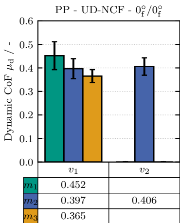
Figure 4.30: Influence of the applied mass m and velocity v on the dynamic CoF for the ply-ply behavior of UD-NCF in a 0^\circ_f/0^\circ_f -configuration.
