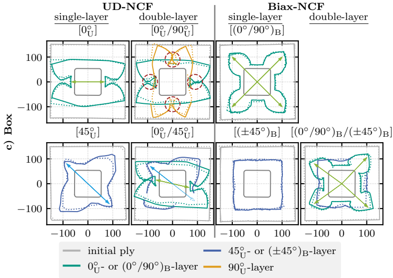
Figure 4.37: Outer contours (all in mm) of single- and double-layer configurations in the box forming tests. Annotations for interactions between layers with arrows and red circles [207].
