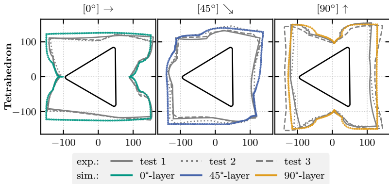
Figure 5.19: Outer contours (all in mm) of the single-layer tetrahedron forming simulations (adapted from [294]).
