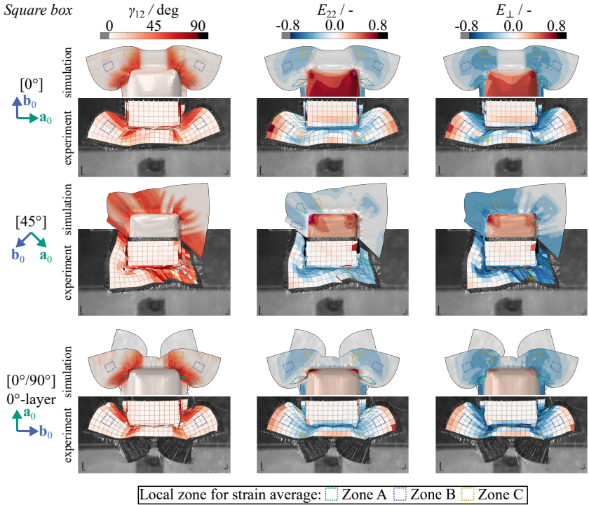
Figure 5.24: Comparison of experimental and simulative strains for [0°] and [45°] single-layer as well as [0°/90°] double-layer setups in the square box forming tests for a punch displacement of u = 85 mm.
