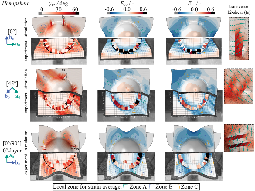
Figure 5.17: Comparison of experimental and simulation strains for [0^\circ] and [45^\circ] single-layer as well as [0^\circ/90^\circ] double-layer setups in the hemisphere forming tests for a punch displacement of u = 75 mm with a zoom on local shear bands due to transverse 12-shear (ts) [294].
