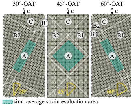
Figure 5.9: Simulation models for the parameterization with off-axis-tension tests (OATs) and highlighted areas (green) for an averaging of the strain components (adapted from [294]).
