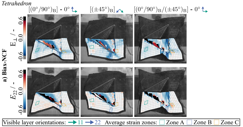
Figure A.8: Additional DIC-strains in the tetrahedron shape forming test from Section 4.6 for Biax-NCF with different layup orientations at a tool displacement of 95 mm [207].
