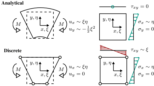
Figure 2.21: Schematic illustration of shear locking for pure bending of a linear quadrilateral elements (based on [307]).
