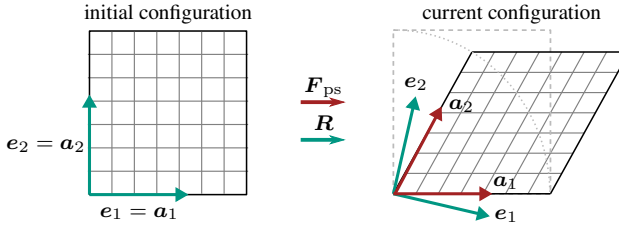
Figure 2.18: Schematic illustration of the rigid body rotation R of the orthogonal Green-Naghdi frame \{e_1, e_2\} and non-orthogonal fiber-parallel frame \{a_1, a_2\} under pure shear deformation F_{ps} .
