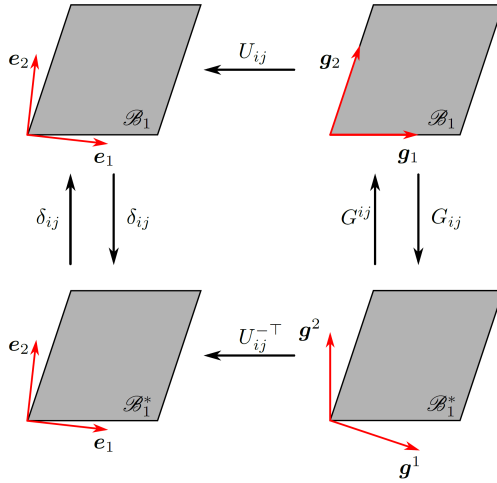
Figure 2.14: Schematic illustration of the transformations in the current configuration \mathcal{B}_1 between Green-Naghdi's frame \{e_i\} and the covariant \{g_i\} and contravariant \{g^i\} fiber parallel frame [17].
