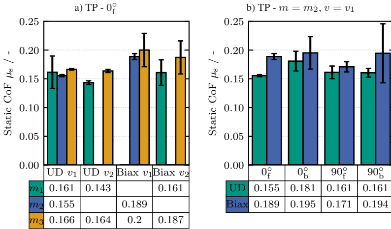
Figure A.4: Experimental results for the tool-ply (TP) static CoF from Section 4.5| (a) Influence of the applied mass m and velocity v in a 0_f^\circ -configuration for both materials; (b) Influence of the relative interface orientations with an applied mass of m = m_2 and velocity v = v_1 .
