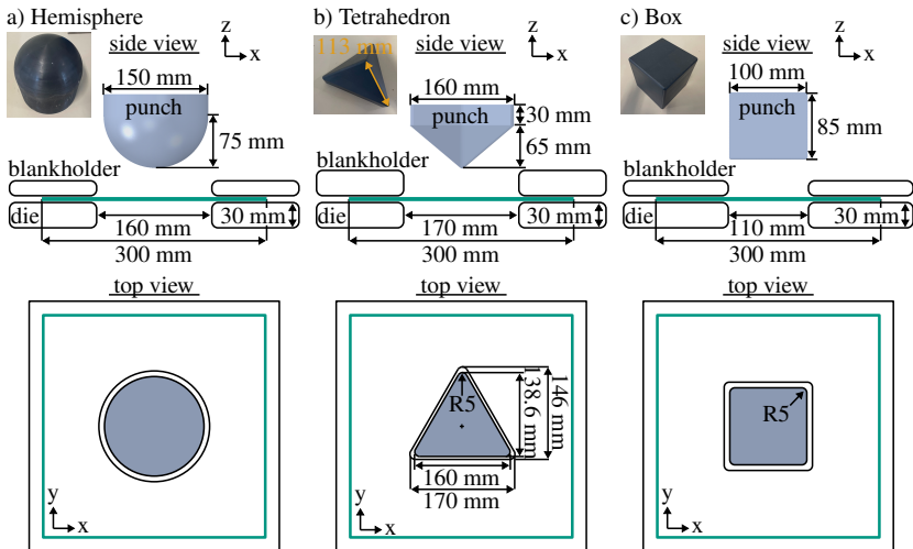
Figure 4.33: Schematics and dimensions of the utilized shapes: a) Hemisphere, b) tetrahedron and c) box [207].
