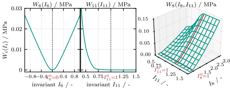
Figure 5.10: Contributions to the strain energy density [294].
