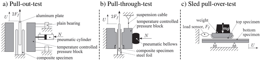
Figure 2.11: Common characterization setups for tangential friction (extracted from [184]).
