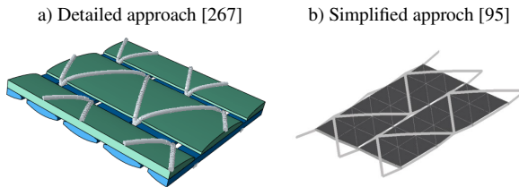
Figure 2.17: Illustration of the different levels of detail in geometrical mesoscopic approaches for a) a Biax-NCF and b) a UD-NCF.
