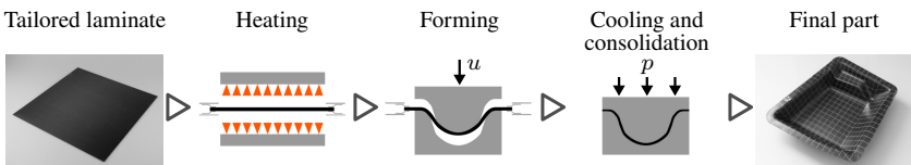
Figure 2.1: Illustration of the different stages in the thermoforming process of a tailored laminate from UD tapes (based on [18]).
