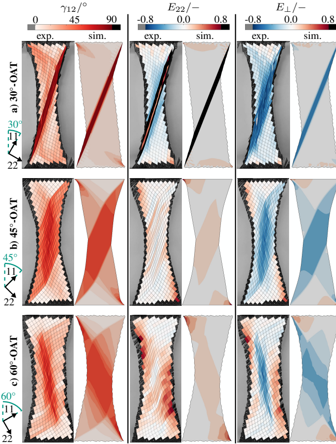
Figure 5.11: Comparison of the experimentally measured (left) and predicted (right) contour plots of the a) 30°-, b) 45°- and c) 60°-OAT at a displacement of 80 mm [294].
