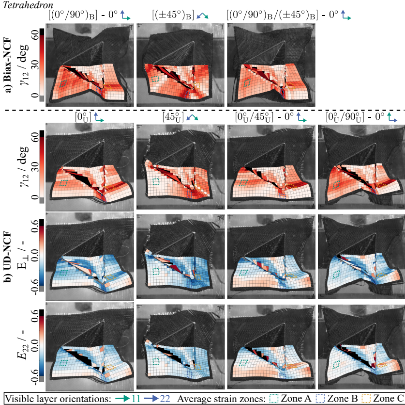
Figure 4.40: Relevant DIC-strains in the tetrahedron shape forming test with different layup orientations at a maximum tool displacement of 95 mm [207].
