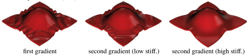
Figure 2.20: Examples for the effect of generalized continua approaches on the a) in-plane behavior of a woven fabric in BET and b) out-of-plane behavior of a thick interlock woven fabric in a hemisphere test.
