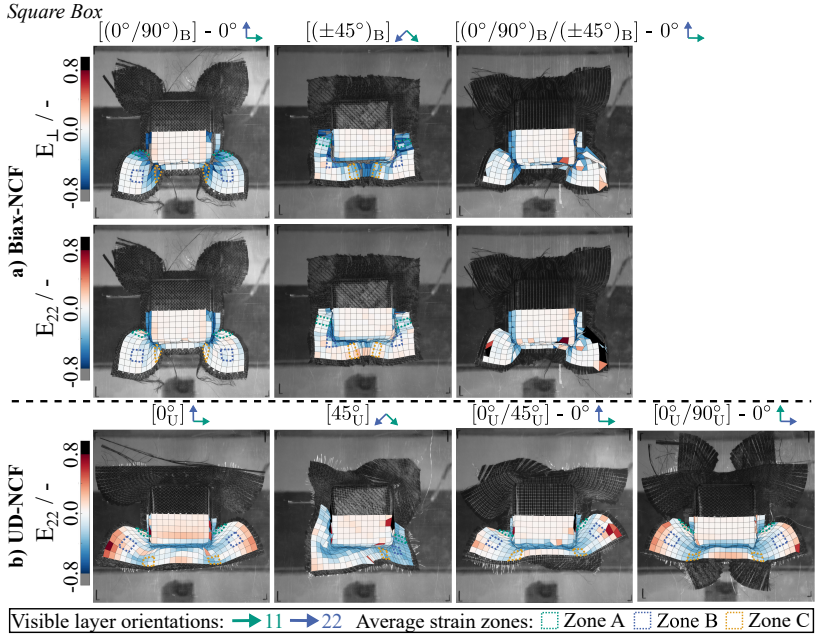
Figure A.9: Additional DIC-strains for the box shape forming test from Section 4.6 for UD- and Biax-NCF with different layup orientations at a tool displacement of 85 mm [207].
