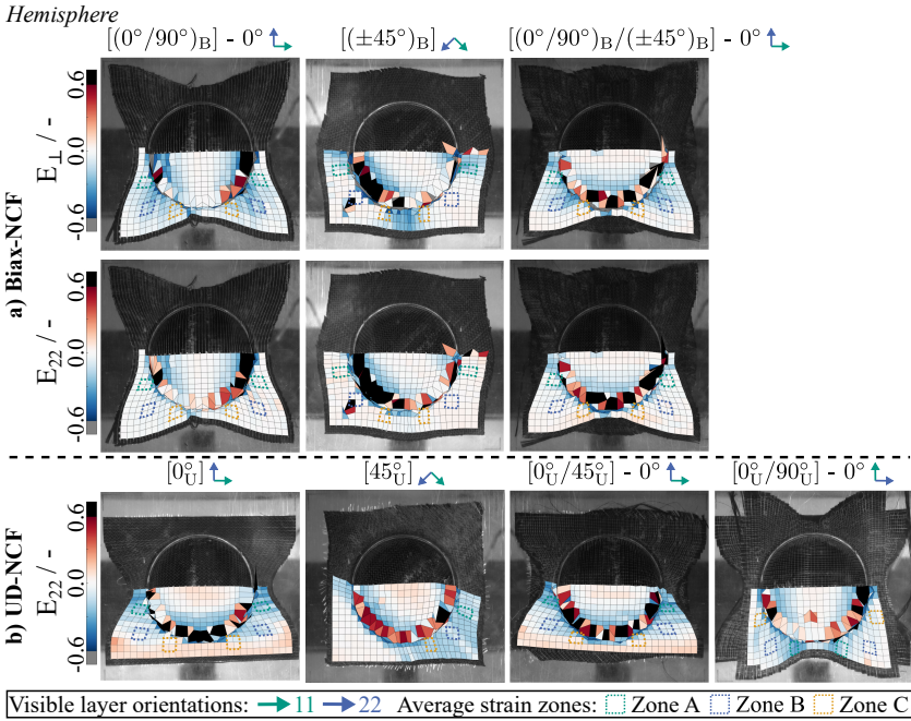
Figure A.7: Additional DIC-strains in the hemisphere shape forming test from Section 4.6 for UD- and Biax-NCF with different layup orientations at a tool displacement of 75 mm [207].
