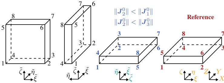
Figure A.17: Schematic illustration of case 2 for a necessary rotation of the COS or node renumbering - First three illustrations represent the initial configuration and necessary rotations - Last illustration represents the desired reference configuration and global COS.
