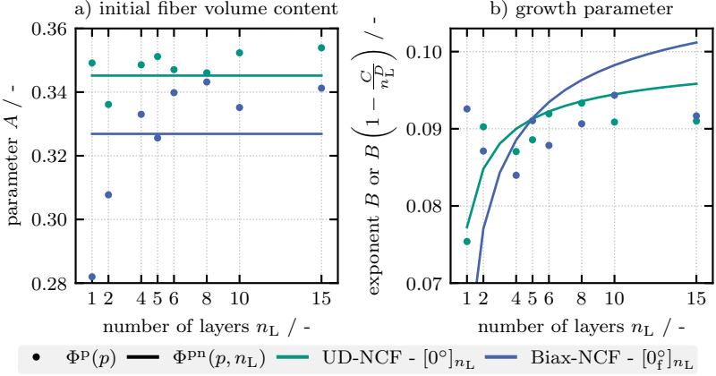
Figure 4.24: Overview of the parameters for the analytical p-model \Phi^P(p) and pn-model \Phi^{pn}(p, n_L) .
