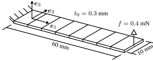
Figure 6.3: Cantilever test setup | Geometry and applied tip load (adapted from [352]).
