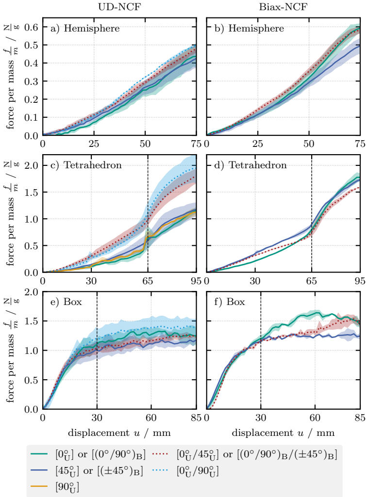
Figure 4.35: Punch forces normalized by the total mass of the fabric layers for the different geometries for Biax- and UD-NCF in single- (solid) or double-layer (dotted) configurations [207].
