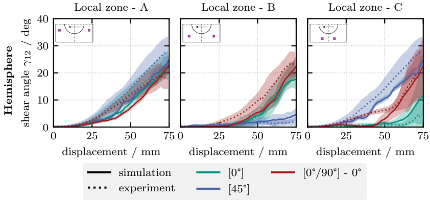
Figure 5.18: Shear angle in local zones of the hemisphere forming tests (adapted from [294]).
