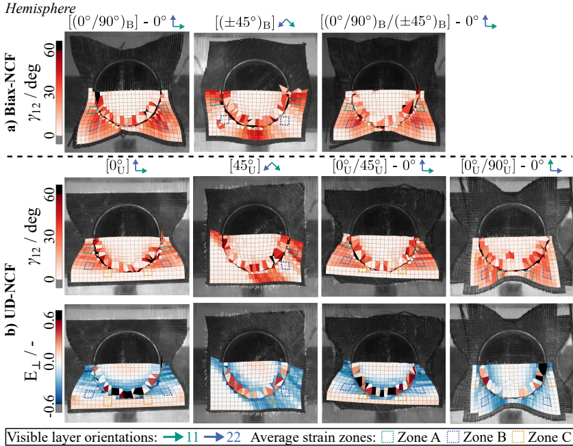
Figure 4.38: Relevant DIC-strains in the hemisphere shape forming test with different layup orientations at a maximum tool displacement of 75 mm [207].
