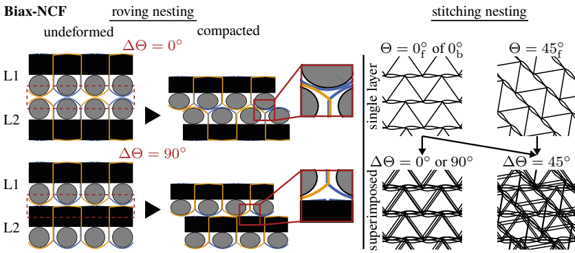
Figure 4.21: Schematic illustration of roving and stitching nesting opportunities for Biax-NCF with a tricot stitching pattern by superposition of multiple cross-sections and stitching patterns.
