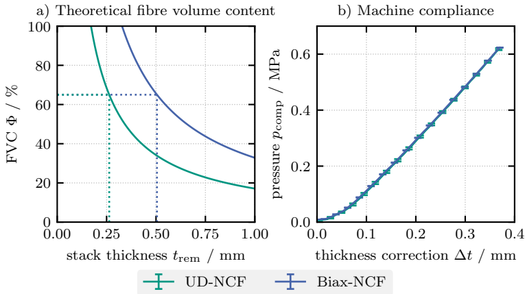
Figure 4.17: (a) Theoretical fiber volume content \Phi for a single layer ( n_L = 1 ) according to Equation 4.7 with dashed lines indicating the remaining thickness t_{\text{rem}} for \Phi = 65\% ; (b) Machine compliance curve during the loading stage (adapted from [167]).
