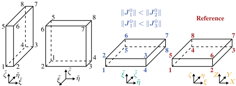
Figure A.16: Schematic illustration of case 1 for a necessary rotation of the COS or node renumbering - First three illustrations represent the initial configuration and necessary rotations - Last illustration represents the desired reference configuration and global COS.
