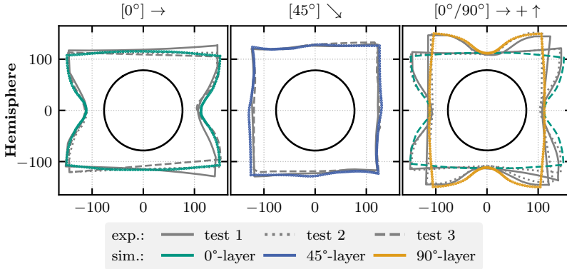
Figure 5.16: Outer contours (all in mm) of the hemisphere forming simulations (adapted from [294]).
