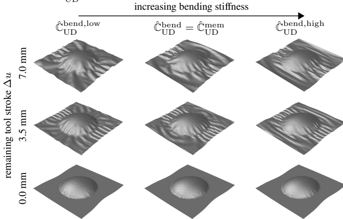
Figure 6.8: Hemisphere forming for different membrane to bending stiffness ratios | Results for a constant a) biaxial and b) unidirectional membrane stiffness with different bending stiffnesses at several remaining tool strokes \Delta u (adapted from [353]).
