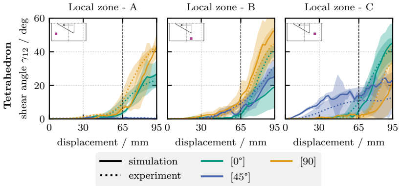
Figure 5.21: Shear angle in local zones of the tetrahedron forming tests (adapted from [294]).
