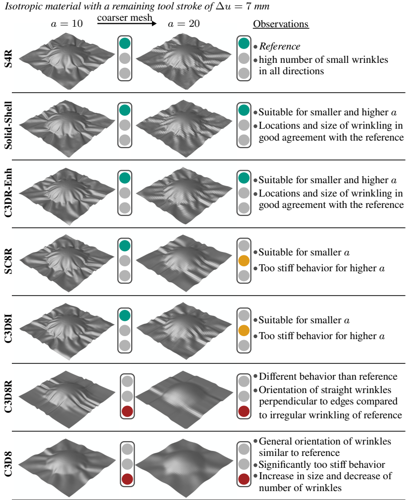
Figure 6.5: Hemisphere forming for isotropic materials | Results and observations for a remaining tool stroke \Delta u = 7 mm for the conventional shell (S4R), solid-shell and different commercially available three-dimensional (C3D8R-Enh, SC8R, C3D8I, C3D8R and C3D8) elements. Colors indicate comparison to S4R-results - green: good agreement; orange: slightly too stiff; red: notable differences (adapted from [352]).
