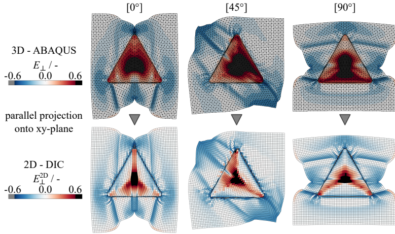
Figure A.14: Exemplary conversion from 3D strains to 2D-equivalent strains by planar projection for the tetrahedron forming simulation in Section 5.4.3.1. [294]
