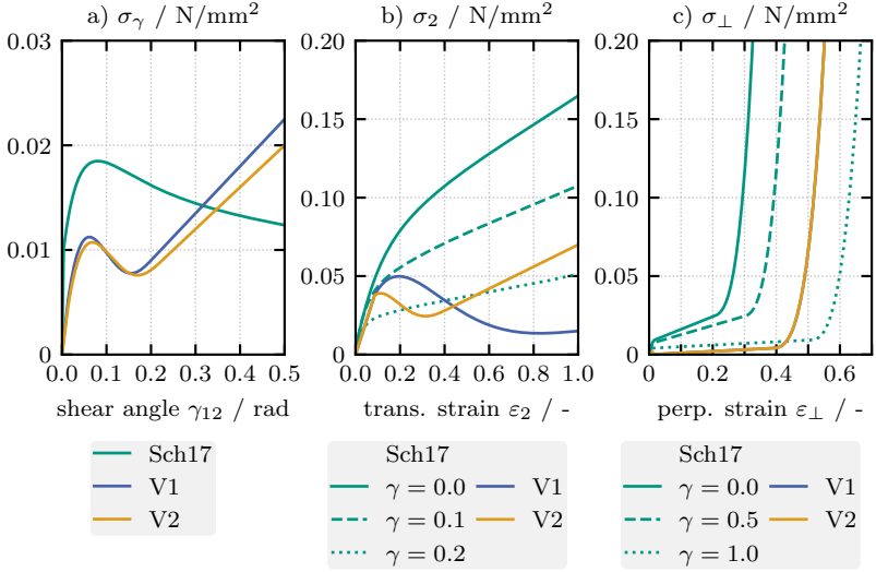
Figure A.10: Equivalent co-rotational stress contributions of the approach by Schirmaier et al. (Sch17) [137] and the decoupled approach from Section 5.1.
