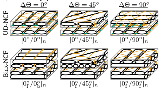
Figure 4.16: (a) Experimental punch-to-plate compaction test setup; (b) Schematic lay-ups of the investigated combinations for different relative fiber orientations at the interfaces with the PES stitching of the NCFs in orange and the GF in green [167].
