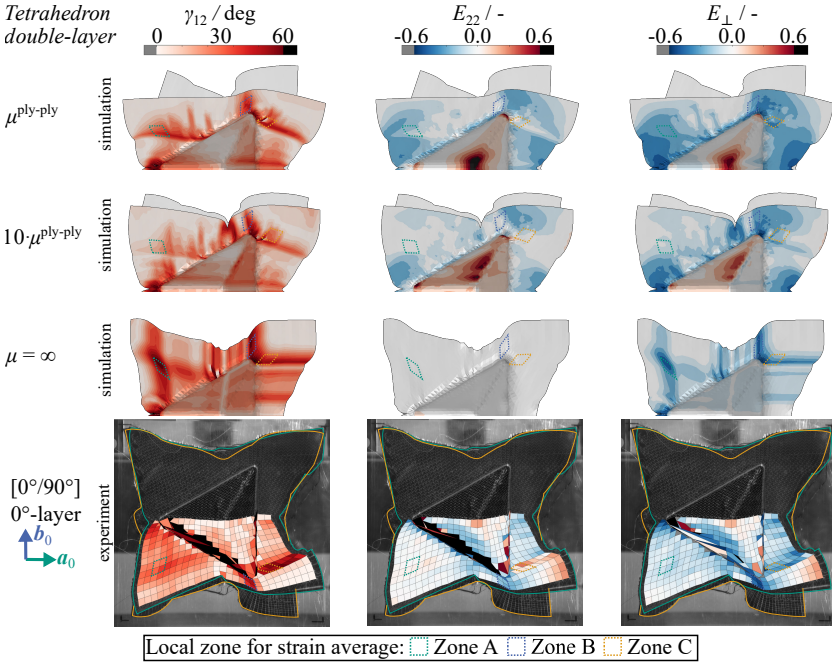
Figure 5.22: Comparison of experimental and simulative strains for [0^\circ/90^\circ] double-layer setups with different ply-ply CoF in the tetrahedron forming tests for a punch displacement of u = 95 \text{ mm}
