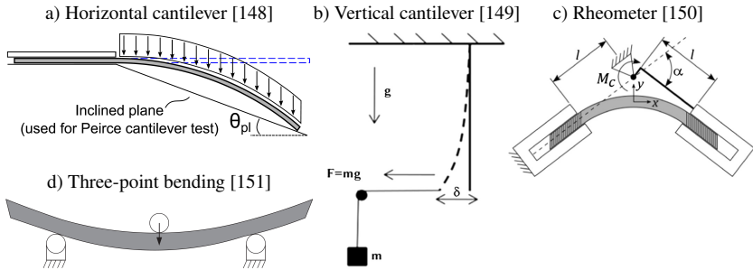
Figure 2.9: Bending characterization setups for engineering textiles
