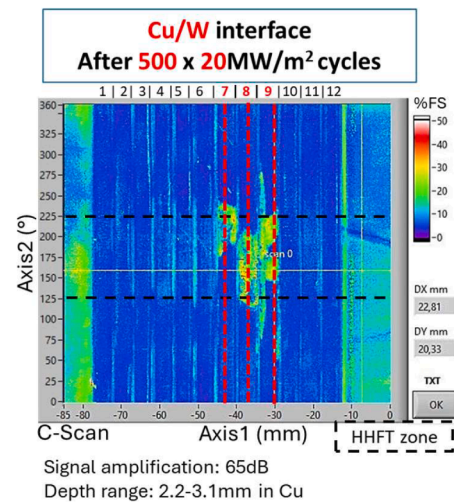
Fig. 11. Cu/W joining interface of MU II -IJS after 500 \times 20\text{MW/m}^2 cycles (2.2–3.1 mm depth range in Cu). A large discontinuity affects the loaded zone of monoblocks #7–8–9. The red dotted lines are circumferential paths used for a more detailed investigation of the morphology and depth of the defect.
