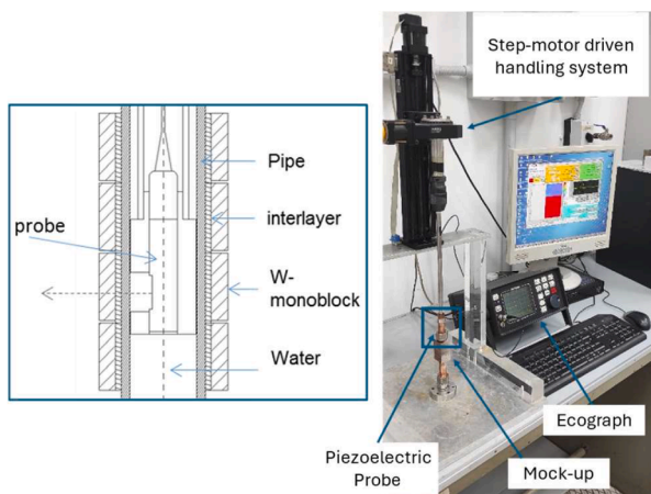
Fig. 2. The employed UT equipment with an axial cross section drawing of the mock-up, showing the probe holder inside the pipe, which ensures the correct probe alignment.
