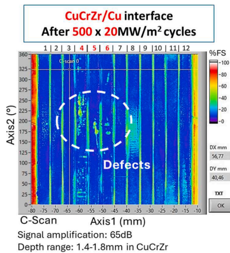
Fig. 10. CuCrZr/Cu joining interface of MU II -IJS after 500 \times 20\text{MW/m}^2 cycles. The presence of clustered discontinuities on monoblock #4–5–6 is highlighted in the C-scan (1.4–1.8 mm depth range in CuCrZr).
