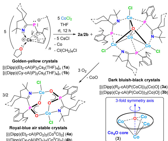
Scheme 1 Syntheses of \text{Co}_4\text{O} clusters 3a–3b [ \text{Co1–Co2} 2.7046(4)], and their reactivity with \text{O}_2 affording dimeric \text{Co}_2^{\text{II}} complexes 4a–4b . 2a–2b are the respective bis- (\text{Dipp})(\text{imino}) -phosphene by-products, isolated separately as white needles (see ESI†).
