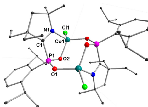
Fig. 2 Molecular structure of [(\text{Dipp})(\text{Et}_2\text{-cAl})\text{PO}_2)_2(\text{Co}^{\text{II}}\text{Cl})_2] ( 4a ). Hydrogen atoms are omitted for clarity. \text{Co2} and \text{O1} have 0.33 occupancy each. The ethyl group ( \text{C9–C10} ) is disordered with a site occupancy ratio of 53:47. Important bond lengths [Å], and bond angles [°]: \text{Co1–Cl1} 2.2034(11) [2.204], \text{Co1–O1} 1.941(2) [1.933], \text{Co1–N1} 2.042(3) [1.912], \text{P1–O2} 1.512(3) [1.554], \text{P1–O1} 1.514(3) [1.539], \text{P1–C1} 1.843(4) [1.824], \text{N1–C1} 1.282(5) [1.296]; \text{O2–P1–O1} 113.39(15) [114.96], \text{P1–O2–Co1} 115.66(15) [116.31].
