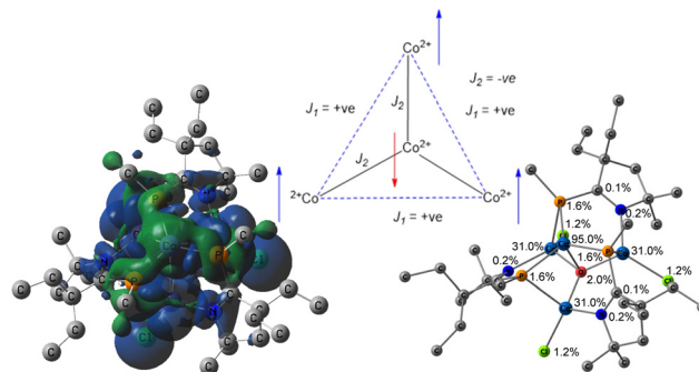
Fig. 3 Mulliken \alpha -(blue), \beta -spin (green) densities of the model complex [(\text{Me})(\text{Et}_2\text{-cAI})\text{P}(\text{CoCl})_3\text{O}] ( 3a' ) at S = 3 (computed at the UB3LYP-D3(BJ)/def2-TZVP level of theory).
