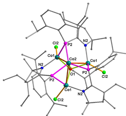
Fig. 1 Molecular structure of the \text{Co}_4^{\text{II}} metal cluster [(\text{Dipp})(\text{Et}_2\text{-cAl})\text{P}(\text{CoCl})_3(\text{CoO})] ( 3a ). Hydrogen atoms are omitted for clarity. Important bond lengths [Å], and bond angles [°]: \text{Co1–Co2} 2.7046(4), \text{Co1–O1} 1.9589(3), \text{Co1–Cl1} 2.2395(5), \text{Co2–O1} 2.036(2), \text{Co2–P1} 2.2808(4), \text{P1–C10} 1.8397(17); \text{C10–P1–Co2} 113.94(6), \text{C10–N1–Co1} 127.76(12). A three-fold axis is present along the \text{Co2–O1} bond.
