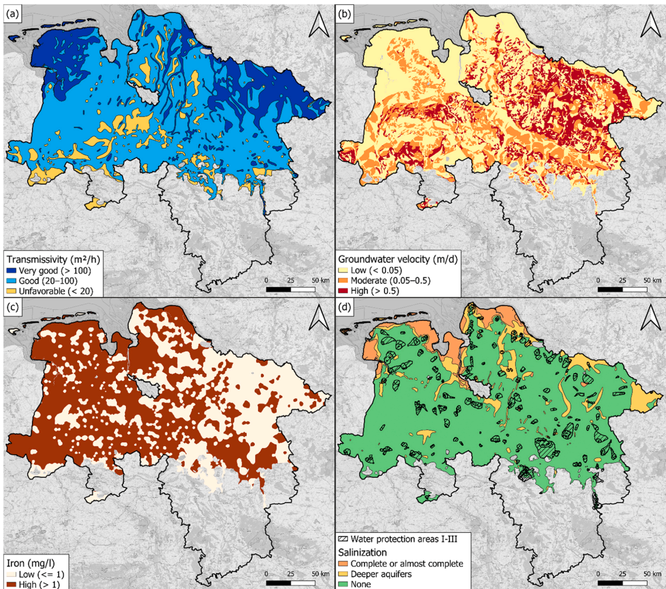
Fig. 1. Spatial distribution of the criteria for the determination of ATE suitability: (a) transmissivity, (b) groundwater velocity, and (c) iron concentration; subplot (d) shows water protection areas and salinized aquifers, which are not considered for ATE suitability determination but are important for legal considerations. Basemap: OpenStreetMap.
