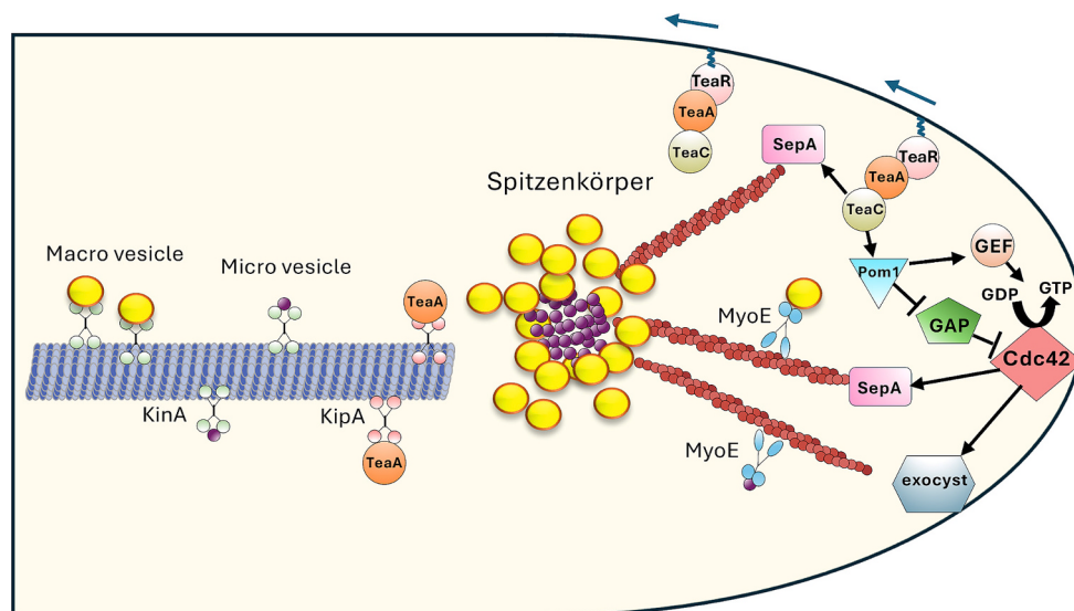
Fig. 4. Interaction of CEMPs with other polarity determinants. Vesicles and CEMPs are transported along microtubules to the tip of a growing hypha. Micro- and macrovesicles accumulate at the Spitzenkörper, where they are distributed to the hyphal tip. The CEMP complex localises at the tip membrane and recruits the formin SepA to promote actin assembly. The following interactions and relations are based mainly on findings in S. pombe and need to be validated in other fungi. Interaction of TeaC and Pom1 may regulate the activity of GAP (GTPase-activating protein) and GEF (guanine nucleotide exchange factor), thereby modulating Cdc42 activation at the site of CEMP localisation. Activated Cdc42, in turn, recruits additional formins and activates the exocyst complex, which is essential for vesicle tethering.
