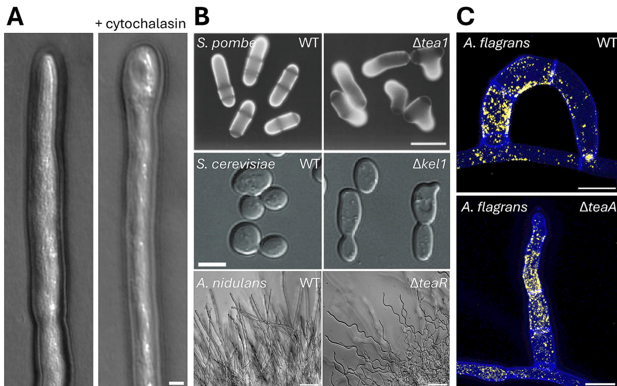
Fig. 1. Cell-end marker proteins (CEMPs) are conserved from yeast to filamentous fungi. A Comparison of a hyphal tip of A. flagrans without and in the presence of cytochalasin A. Scale bar, 2 μm. B Deletion of CEMP encoding genes in S. pombe , S. cerevisiae , and A. nidulans . C Trap morphology in A. flagrans and the \Delta teaA mutant. To demonstrate that both structures are physiologically traps, the trap-specific, small-secreted protein, NipA, is visualised as a RFP-fusion protein (yellow) (Emser et al., 2024). Pictures in B and C were taken from (Mata and Nurse, 1997; Kriegler et al., 2025; Garcia et al., 2021). (For interpretation of the references to colour in this figure legend, the reader is referred to the web version of this article.)
