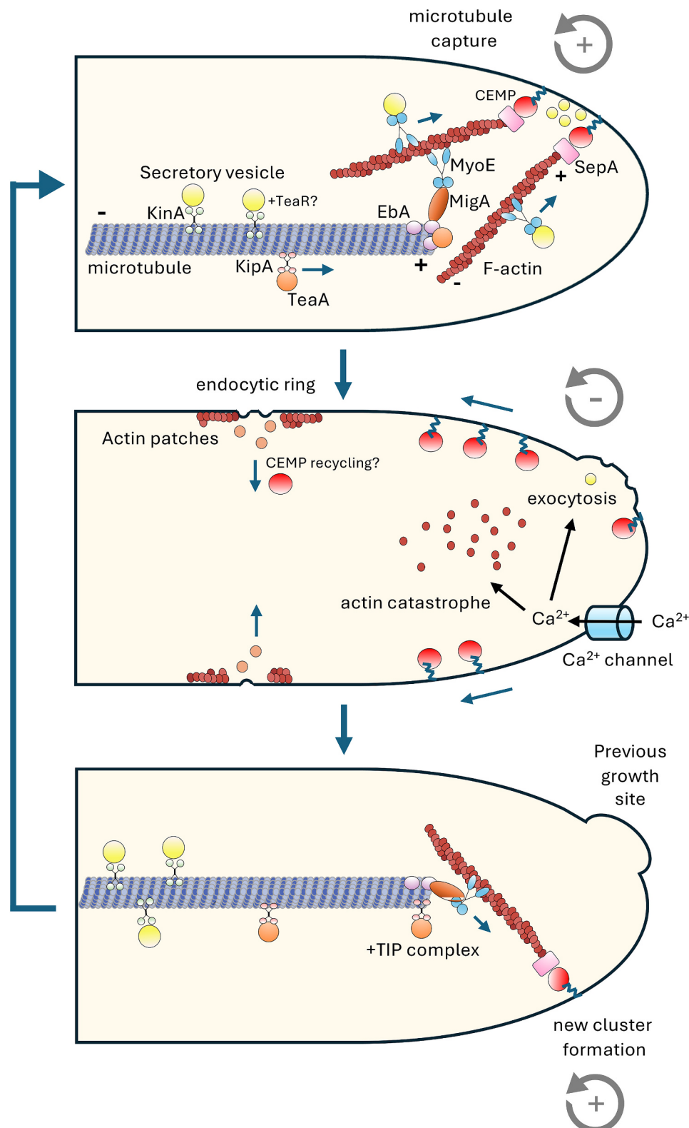
Fig. 3. Role of CEMPs in establishment of local growth sites. Upper panel: CEMPs are transported along microtubules either directly as cargo of the kinesin VII KipA (TeaA), or in the case of the prenylated TeaR receptor at vesicles. KipA and TeaA accumulate at microtubule plus ends and are thus microtubule plus end tracking proteins (+TIP). A small CEMP complex at the membrane assembles actin filaments along which microtubule plus ends are pulled to merge at one point and deliver more CEMPs. This leads to more actin filaments. Secretory vesicles are transported along microtubules with conventional kinesin as a motor before they are reloaded onto actin filaments. Vesicles containing cell-wall biosynthesis enzymes accumulate around the CEMP site. Middle and lower panels: Pulsed Ca 2+ influx induces fusion of the secretory vesicles with the membrane and actin catastrophe. The cell wall will be synthesised at that place. Membrane integration disturbs the integrity of the CEMP complexes, which then dissolve. Some of them will be internalised in the endocytic ring, and others give rise to new actin filament formation.
