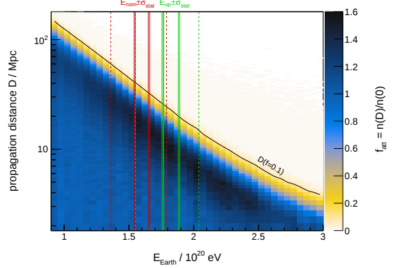
Figure 4: Propagation distances of CRs arriving at Earth, in each bin of energy as given on the x-axis of the plot, for iron injected with an \mathcal{R}_{\text{max}} = 10^{18.6} V energy spectrum (see text for details)
