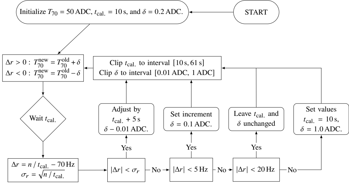
Figure 4: Flowchart describing the rate-based algorithm to approximate I_{MIP} independently on an LS. The idea and implementation details are based on a rate-based calibration of the WCD PMTs as explained in [5].
