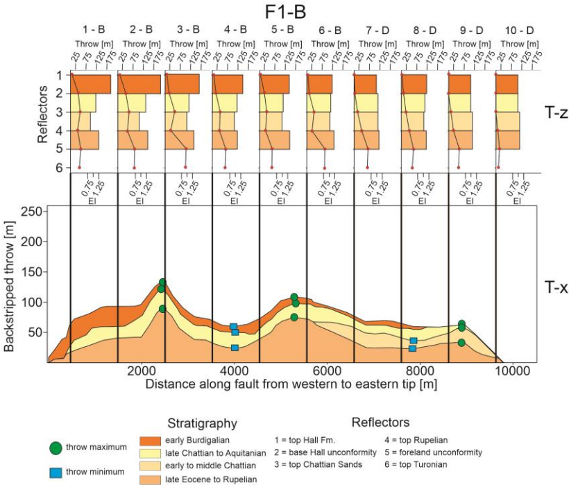
Figure 3.6: Backstripped T-x profile with 10 T-z profiles along the length of fault F1-B. El values of the different seismic-stratigraphic units are given in coloured boxes in the T-z profiles.
