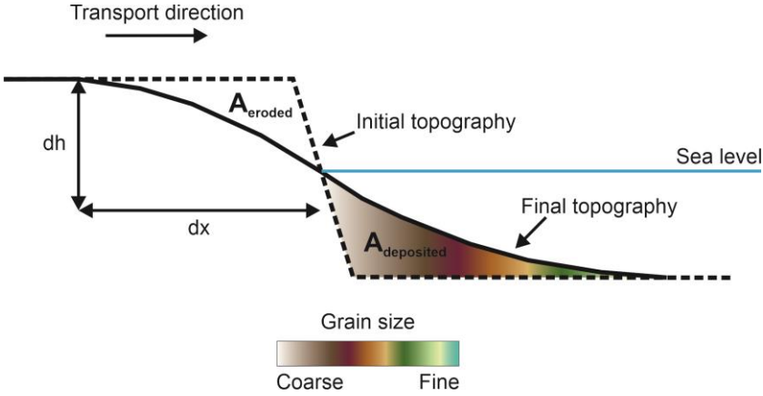
Figure 5.1: Schematic representation of diffusion in GPM of multiple sediment types. A_{eroded} is the area of the initial topography that is eroded after time increment dt , and is equal to the area A_{deposited} downslope.
