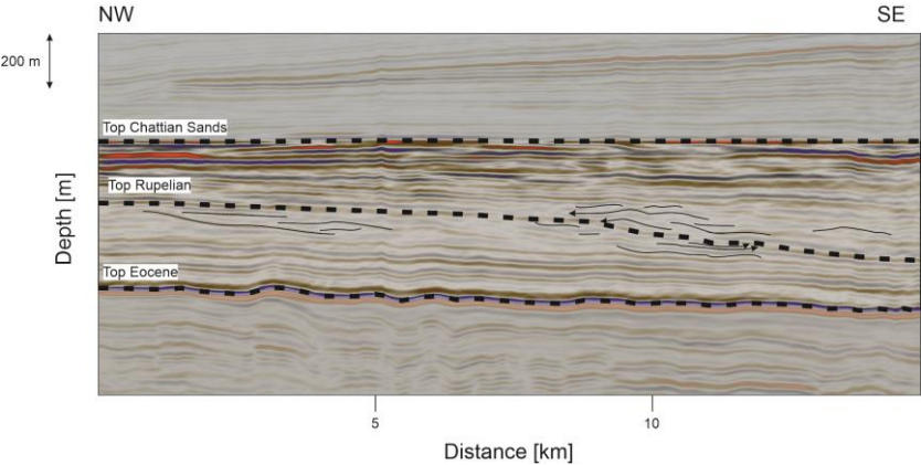
Figure A1.6: SE dipping Clinoforms (black solid lines) in the Upper Rupelian and Lower Chattian seismic stratigraphy. Arrows indicate reflector terminations.
