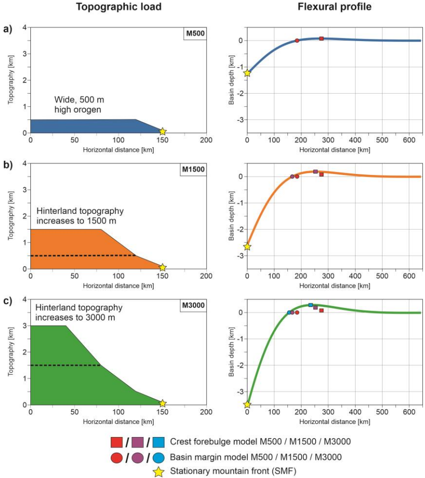
Figure 4.5: Three different scenarios of topographic load distribution in the orogen and respective flexural profile for models a) M500, b) M1500, and c) M3000. For the topographic loads, the coloured area above the dashed line represents the added topographic load from model M500 to model M1500 and from model M1500 to model M3000 in figures b and c, respectively.
