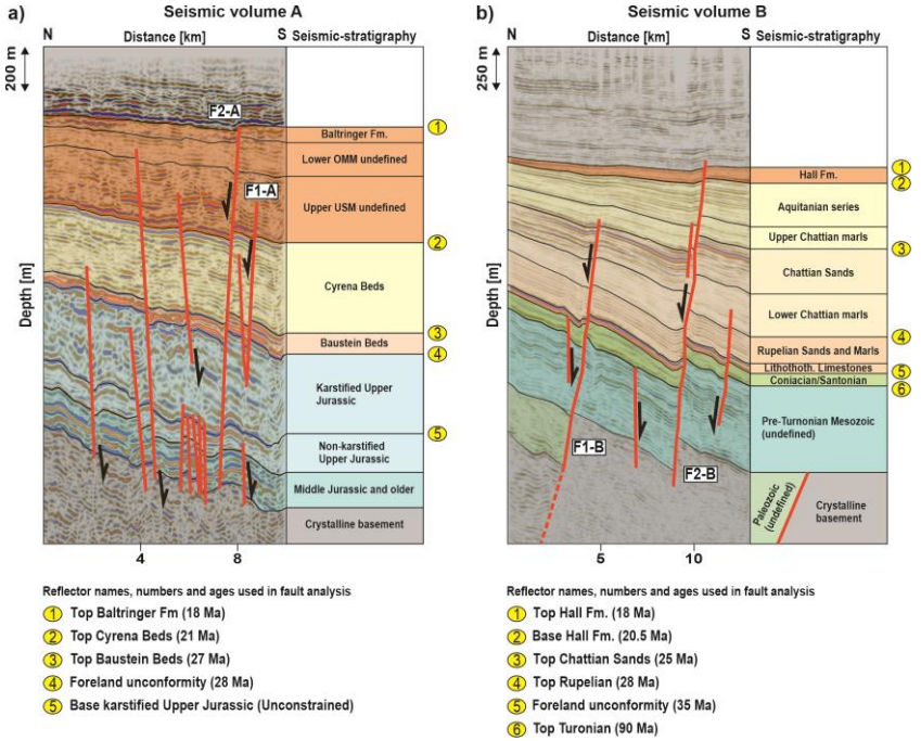
Figure 3.3: a) Seismic stratigraphy in seismic volume A west of Munich, based on Eskens et al. (2024). The ages of reflectors are based on Kuhleermann and Kempf (2002), von Doppler et al. (2005), Heimann et al. (2009), Heckeberg et al. (2010), and Shipilin et al. (2020). USM = Upper Freshwater Molasse. b) Seismic stratigraphy in seismic volume B east of Munich, based on Eskens et al. (2024). The ages of the different reflectors are based on Jin et al. (1995) and Zweigel et al. (1998). Unconstrained means the age of the reflector is unknown. Reflector numbers are the same as in Figures 3.5 (Volume A), 3.6 and 3.7 (Volume B). Not numbered reflectors are not included in the fault analysis due to poor traceability. Unconstrained means the exact age of the reflector is unknown, and the unlabelled reflectors are not included in the fault analysis due to poor traceability in the entire seismic volume.
