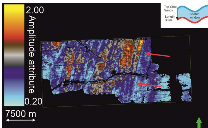
Figure 1.11: Sweetness map of the Middle Chattian seismic stratigraphic unit. High amplitudes indicate more sandy areas, low amplitudes indicate more muddy areas. As such, the NE-SW bands of high and low sweetness values are interpreted to highlight the orientation of an NE-SW directed coastline. The western side was a more shallow and sandy area. In contrast, the eastern side is more mud-rich and was likely located in a deeper water depositional environment. Red arrows indicate the direction of onlap.
