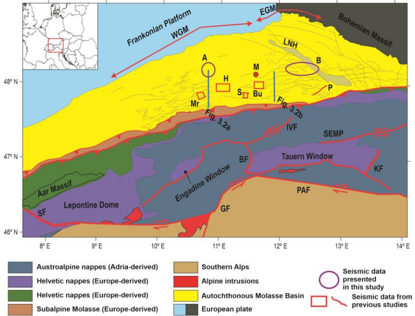
Figure 3.1: Map of the major tectonic units in the Alps, modified from (Schmid et al., 2004a). Thin black lines in the Molasse Basin indicate the locations of syn-flexural normal faults, based on the GeoMol project, (Mraz et al., 2018), and (Freudenberger and Schwerd, 1996). A : seismic volume A, B : seismic volume B, LNH : Landshut-Neuoetting High, BF : Brenner Fault, PAF : Periadriatic Fault, KF : Katschberg Fault, GF : Giudicarie Fault, IVF : Inntal Valley Fault, SF : Simplon Fault. Locations of previous studies: Bu : (Budach et al., 2018), H : (von Hartmann et al., 2016), Mr : (Mraz et al., 2018), P : (Cordero Peña, 2007), S : (Shipilin et al., 2020).
