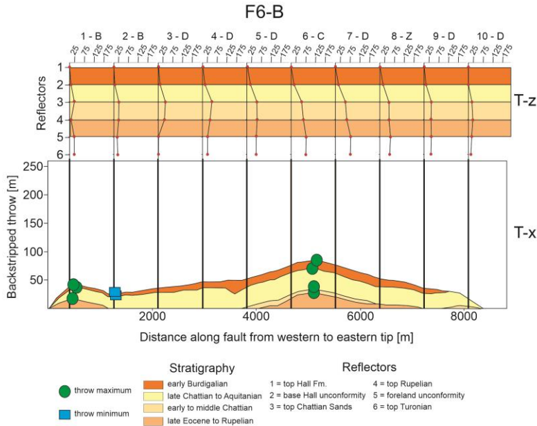
Figure A2.5 (continued): T-x profile with 10 T-z profiles along the length of fault c) F6-B.
