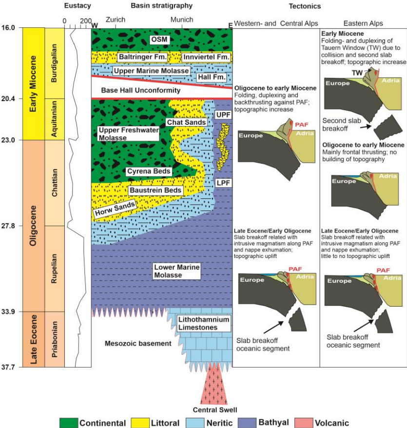
Figure 6.1: Schematic west-east Wheeler diagram of the syn-orogenic fill of the Molasse Basin and the respective depositional environments it represents, as well as coeval eustacy and litho-spheric processes. The basin west of Munich defines the Western Molasse, the basin to the east of Munich the Eastern Molasse. Inspired by Kuhlemann and Kempf (2002), their Figure 2. The tectonics pane highlights which processes were fundamental forcing the underfilled to overfilled transition in the Western- and Eastern Molasse, respectively.
