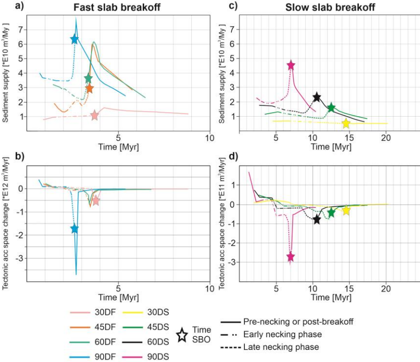
Figure 5.8): a) Sediment supply rate changes for fast breakoff models. The dashed sections of the curves indicate ongoing slab necking. b) Volume of accommodation space being generated (positive values) or destroyed (negative values) due to tectonics for the fast slab breakoff models. c) Sediment supply rate changes for slow breakoff models. The dashed sections of the curves indicate ongoing slab necking. d) Volume of accommodation space being generated (positive values) or destroyed (negative values) due to tectonics for the slow slab breakoff models. SBO = slab breakoff.
