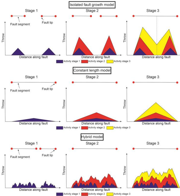
Figure A2.1: Conceptual model for lateral (along-strike) normal fault growth signature in T-x graphs for the isolated, constant length and hybrid fault growth models. For the isolated fault growth model, lateral growth occurs through tip migration and subsequent linkage of previously separated fault segments. Modified from (Hongxing and Anderson, 2007; Peacock and Sanderson, 1991; Ryan et al., 2017; Wang et al., 2022). For the constant length model, the final length of the fault is established during the early stages of fault development, accumulating offset along the entire fault over time (Jackson et al., 2017; Jackson and Rotevatn, 2013; Walsh et al., 2002). The hybrid model combines of the isolated- and constant-length growth models. In this case, the early stage is defined by the lengthening of the fault, laterally linking along (most of) its length. Subsequently, offset accumulates along the fault coeval with minor lengthening (Jackson et al., 2017).
