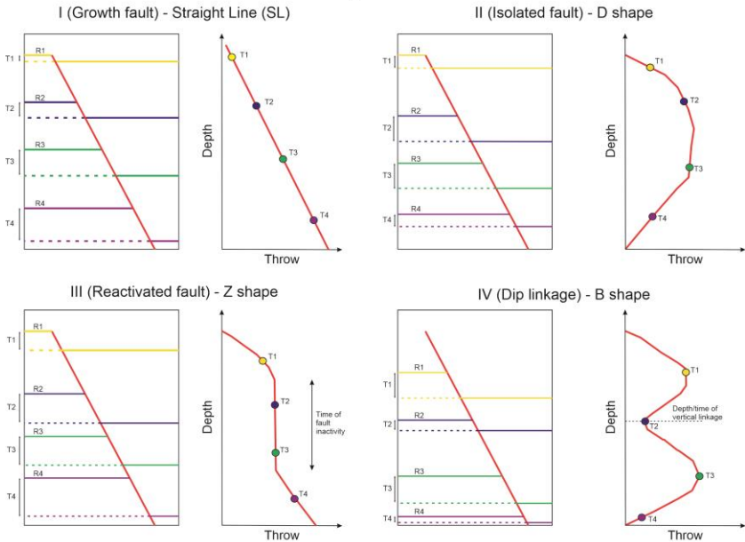
Figure A2.2: Conceptual models for down-dip (vertical) normal fault growth signature in T-z graphs. Assuming the entire fault surface is active during phases of tectonic activity, the stratigraphic surface which records the highest offset indicates the time and point of initial nucleation. (I) A growth fault nucleates at depth, growing continuously upward in the stratigraphy. In a T-z graph, this is recognised as an upward continuous decrease in offsets compared to the lowest stratigraphic surface (Hongxing and Anderson, 2007; Ryan et al., 2017). (II) An isolated fault nucleates in the middle of a stratigraphic sequence, subsequently propagating both down- and upward in the stratigraphy. This is recognised in a T-z graph as the highest offset being recorded midway down the fault, decreasing both down- and upward (Hongxing and Anderson, 2007), giving the T-z profile a D-shape. (III) A reactivated fault nucleates at depth, subsequently becoming inactive before being reactivated during a 2 nd phase of activity. In a T-z graph, this is recognised as the maximum throws being observed for the deepest stratigraphic surface, remaining constant for a few surfaces before subsequently decreasing for the youngest stratigraphy cut by the fault (Ryan et al., 2017), giving the T-z profile a Z-shape. (IV) A vertically dip-linked fault initially consisted of two mechanically separated segments which linked as both faults grew down- and upward. In a T-z graph, this is reflected by two throw maxima at different depths with decreasing offsets both down- and upward. Between the throw maxima, a throw minimum indicates the vertical linkage position (Baudon and Cartwright, 2008). Overall, this gives the t-Z profile a B shape. Modified from (Wang et al., 2022).
