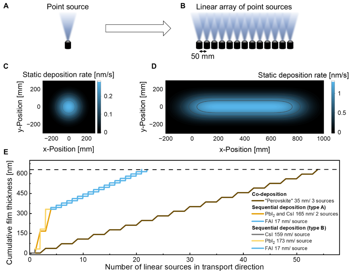
Fig. 5 A/C Schematic and spatial static deposition rate of a point source, exemplary shown for FAI. B/D Schematic and spatial static deposition rate of a linear source, exemplary shown for FAI. E Number of linear sources required in parallel to achieve a cumulative film thickness of 630 nm (30 nm CsI, 300 nm \text{PbI}_2 and 300 nm FAI). The substrate speed is set to 1 \text{ m min}^{-1} , therefore the deposited film thickness per source equals its dynamic deposition rate in \text{nm m min}^{-1} (see Fig. S14).
