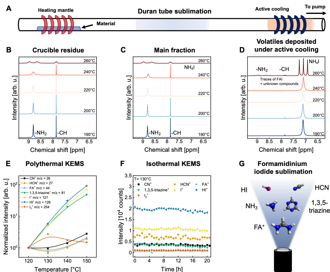
Fig. 2 Investigation of the thermal stability of FAI under sublimation conditions A Schematic drawing of the employed sublimation setup used. Material is collected from the crucible residue, the main fraction, and the volatiles deposited under active cooling. B-D ^1\text{H-NMR} spectra of collected material for increasing sublimation temperatures E KEMS measurements of pristine FAI with increasing temperature. Lines are guides for the eye. F Isothermal KEMS measurements at 130 °C. G Graphical summary of species emitted from the sublimation source.
