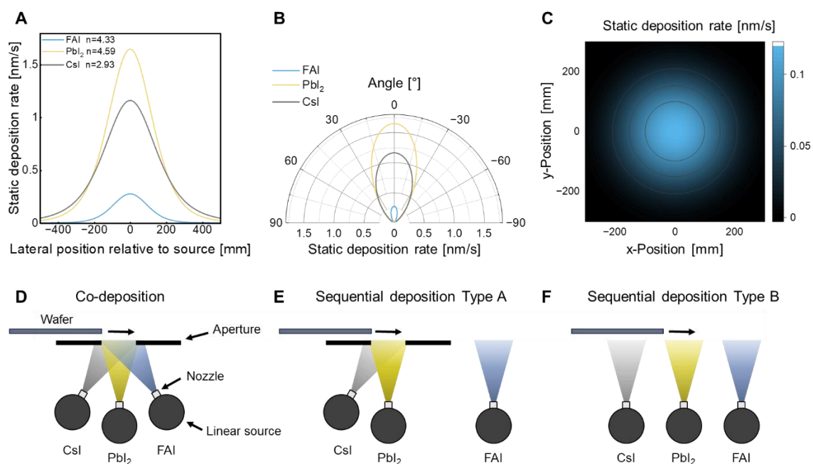
Fig. 4 Vapor cloud shape of relevant perovskite precursors and transfer of deposition modes to linear source setup A/B Static deposition rate as a function of the position relative to the source of the considered perovskite precursor materials (PbI 2 , FAI
