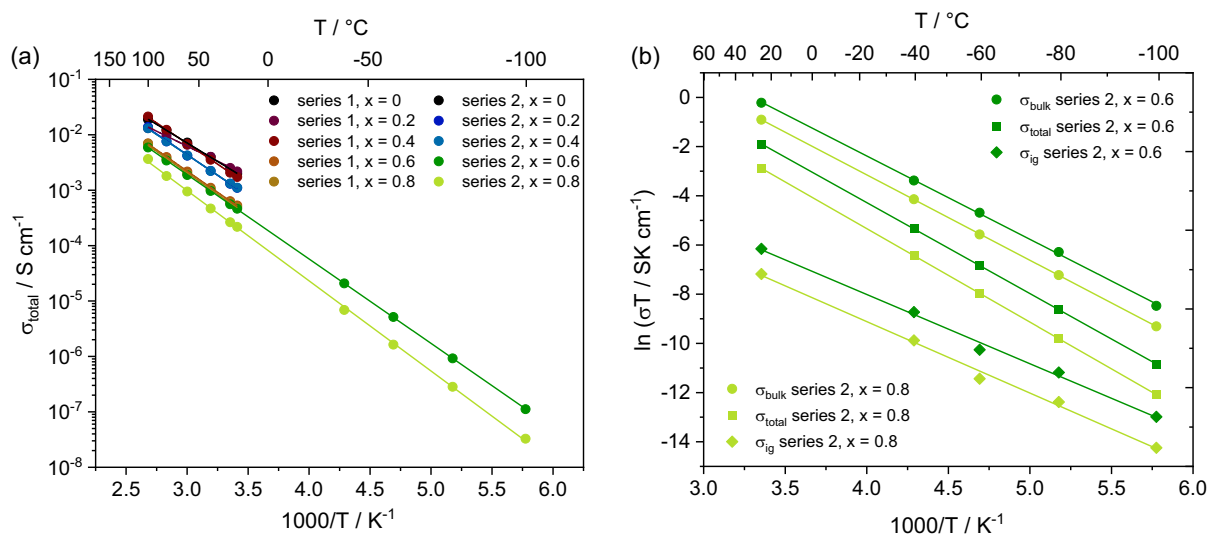
Figure 4. a) Temperature-dependent measurements in the temperature range of -100 – 100^\circ\text{C} . b) Low-temperature data between 20^\circ\text{C} and -100^\circ\text{C} for the samples of CS2 with the highest glass content ( x = 0.6 and x = 0.8 ). Very noteworthy, the slope of \sigma_{\text{ig}} is significantly lower than those of \sigma_{\text{bulk}} and \sigma_{\text{total}} .
