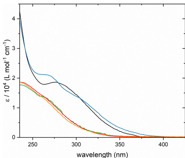
Fig. 3 UV-vis spectra collected in DCM at room temperature of [\text{Cu}(\mu\text{-trz})(\text{NP})_2] (black line), [\text{Cu}(\mu\text{-trz})(\text{NP}^{\text{F}})]_2 (orange line), [\text{Cu}(\mu\text{-trz})(\text{NP}^{\text{Ar}})]_2 (green line), [\text{Cu}(\mu\text{-trz})(\text{NP}^{\text{PyR}})]_2 (red line) and [\text{Cu}(\mu\text{-trz})(\text{N}_{\text{PyP}})]_2 (blue line).
