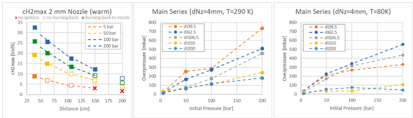
Fig. 5. Left: combination of cH 2 -measurements (dashed lines) and combustion behavior (symbols). Center and right: examples for maximum measured overpressures in experiments at ambient and cryogenic temperature [104].
