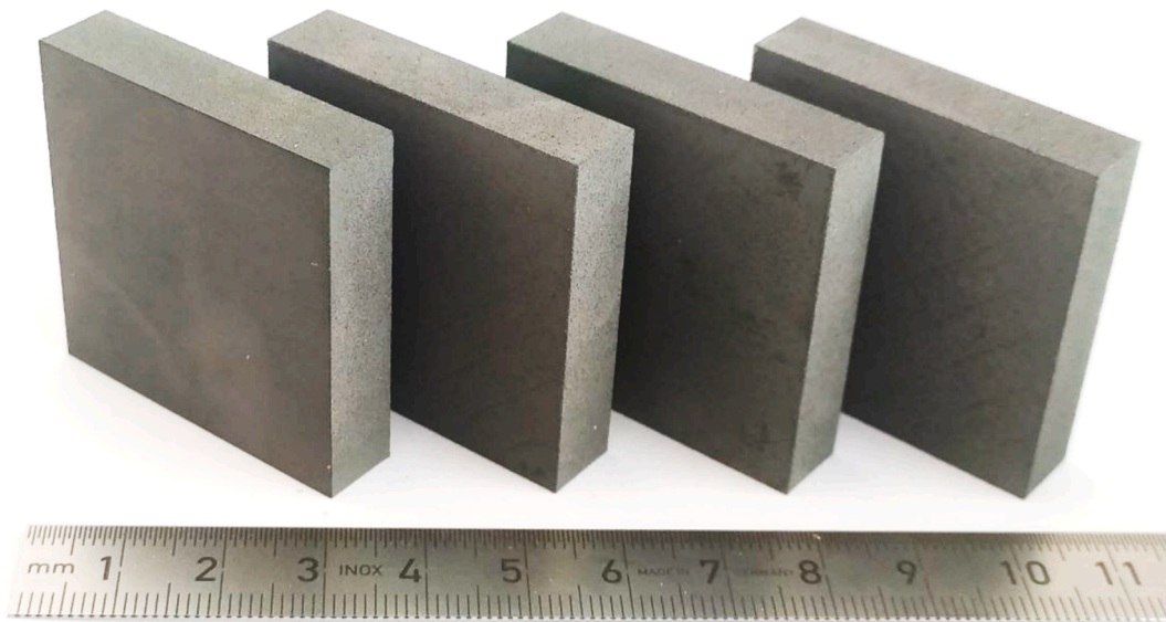
Fig. 2. Appearance of the as-received SLM-EF blocks, Fabrication 2 ( 40 \times 40 \times 10 \text{ mm}^3 ), produced via selective laser melting.
