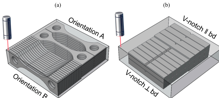
Fig. 1. Schematic of specimens cutting for (a) tensile and (b) Charpy impact tests.
