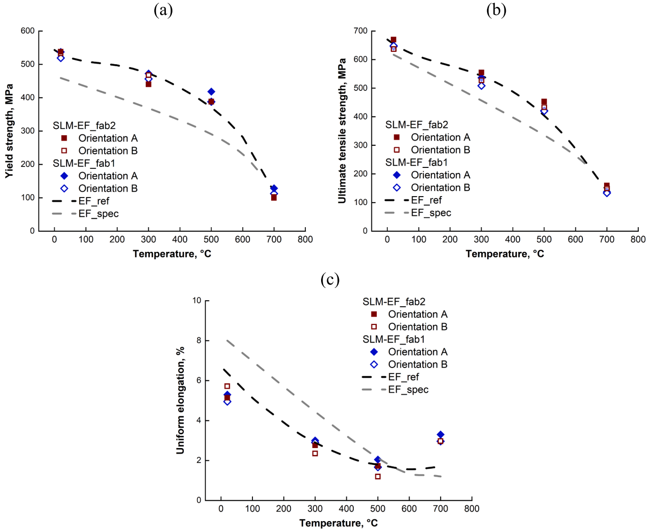
Fig. 4. Tensile test results for SLM-EF from fabrications 1 and 2 at temperatures of 20, 300, 500, and 700 °C: (a) yield strength, (b) ultimate tensile strength, and (c) uniform elongation. The materials were evaluated in two orientations: Orientation A, where samples were aligned parallel to the powder layers, and Orientation B, perpendicular to the powder layers. The tensile properties of the reference material EUROFER97 (EF_ref), and data from literature for EF_spec are presented as dashed lines for comparison [12,19–22]. Standard deviations are typically within \pm 3 % for strength values, \pm 15 % at 20–300 °C, and \pm 40 % at 500–700 °C for elongation.
