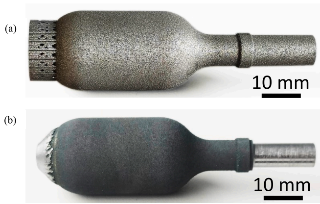
Fig. 7. Burst capsules of SLM-EF in the (a) as-printed state and (b) after HIP, heat treatment, and partial lathe processing.
