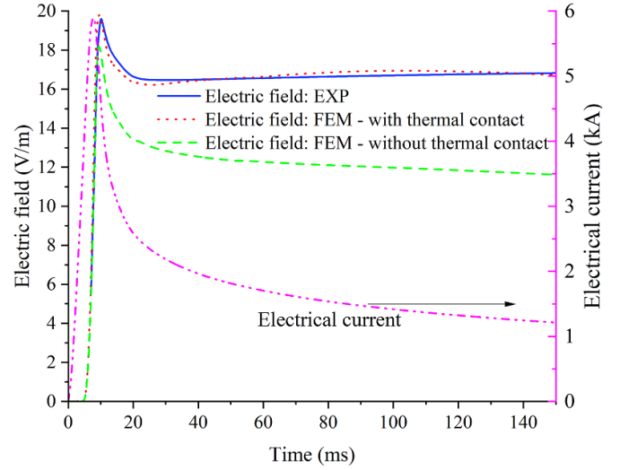
Figure 3. The electric fields and electrical current in the cable during a 150 ms fault for which the transport current surges to about nearly twice the cable critical current.
