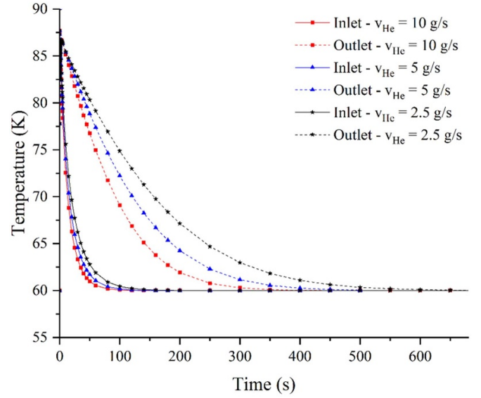
Figure 20. Evolution of temperature of the innermost layer at the inlet and outlet locations for different helium gas flow rates.
