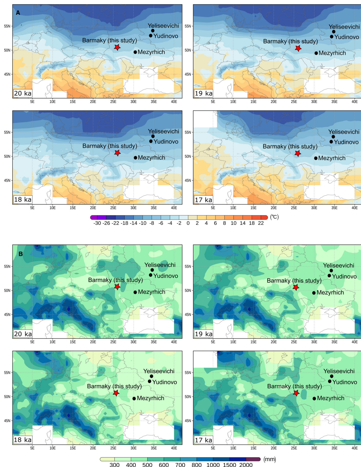
Fig 4. Modelled climatic development. A. Mean annual air temperature (MAAT in °C). B. Mean annual precipitation sum (MAP in mm) from the time period 20–17 cal. ka BP in central Europe. White, spared parts represent large water bodies.
