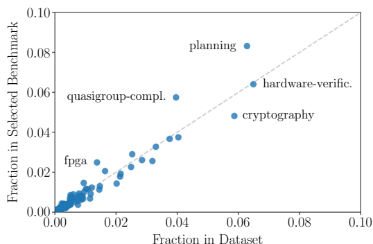
Fig. 7 Scatter plot illustrating the relative importance of different instance families for ranking on the full dataset. The x-axis depicts the frequency of instance families in the dataset, while the y-axis represents the average frequency in the samples selected by active learning. The dashed line represents families that occur with the same frequency in the dataset and samples. Results are on the full dataset with cross-validation over all solvers
