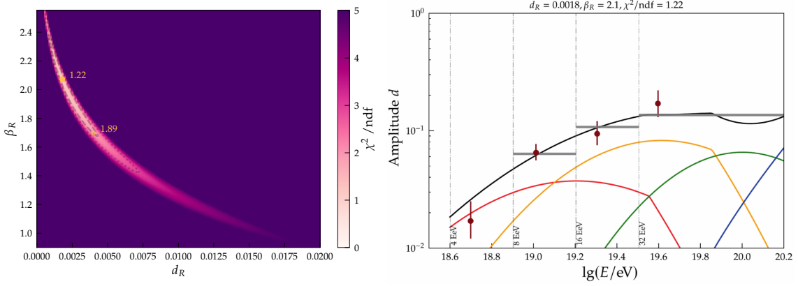
Figure 3: Left: maps of reduced \chi^2 for the possible parameters in Eq. (1). The \chi^2 is a goodness-of-fit evaluation of these parameters to describe the measured dipole amplitudes from Ref. [4] in each energy bin. The expected dipole amplitude in each energy bin is computed via Eq. (1), and the contribution from each component follows the composition fraction as described in the EPOS extended Auger mix, weighted by the spectrum function. The maximum dipole amplitude considered here is d_{\max} = 3 . Contours denote points with \chi^2/\text{ndf} = 2 (dashed line) and with \chi^2/\text{ndf} = 3 (dotted line). A full circle denotes the best parameters for the EPOS extended Auger mix composition, while the empty star denotes an edge point, falling just within the \chi^2/\text{ndf} = 2 contour region with d_R = 0.004 and \beta_R = 1.7 . Right: contribution to the dipole amplitude by each component: proton (red), helium (orange), CNO (green), and iron (blue). Summing all contributions, the total dipole amplitude is shown in black. Horizontal gray bars correspond to the spectrum-weighted total dipole amplitude in each large energy bin. Dark red markers represent the measured dipole amplitude as in Ref. [4]. The parameters that allow for the best description of the data, denoted with a circle in the left-side graph, are used in this realization and correspond to d_R = 0.0018 and \beta_R = 2.1 .
