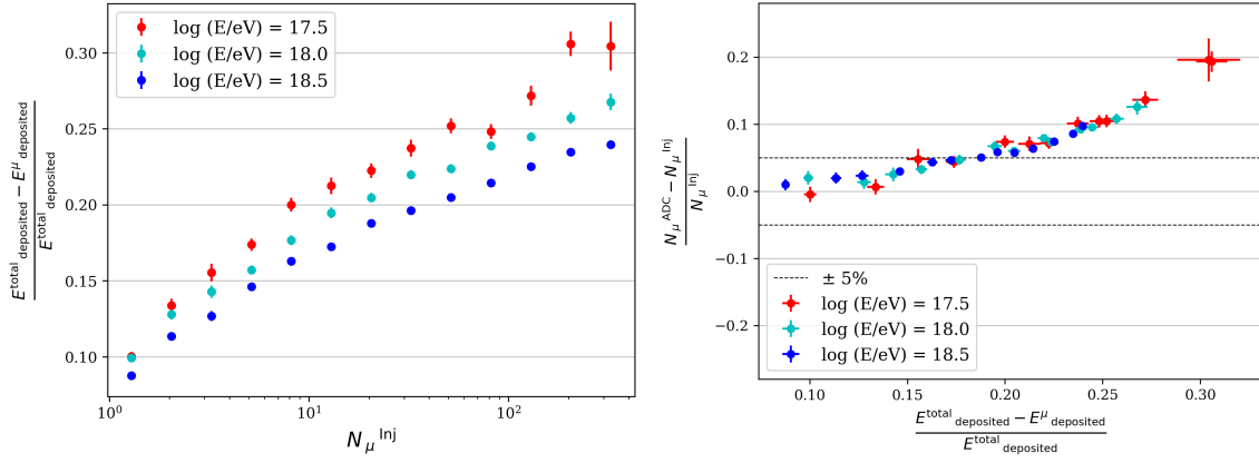
Figure 7: (left) Fraction of energy deposited by particles excluding muons as a function of the number of injected muons per 10 m 2 module. (right) Bias in the muon reconstruction of the ADC mode as a function of the fraction of the energy deposited by particles other than muons.
