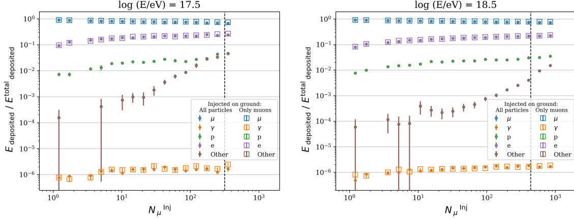
Figure 6: Fraction of energy deposited by the different types of particles as a function of the number of injected muons per 10 m 2 module, for the two sets of simulations: all particles injected into the ground (filled circles) and only muons (unfilled rectangles). A dashed line denotes a rough estimate of the saturation.
