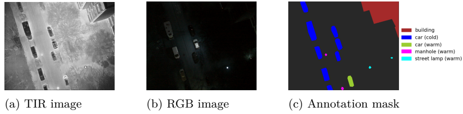
Fig. 1: Example of a multispectral image from the dataset, consisting of RGB and TIR, as well as associated annotation mask. Figure based on [38].
