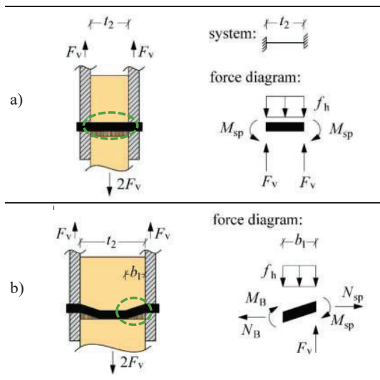
Figure 2: Force diagrams for two possible failure modes:
