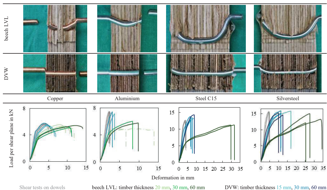
Figure 3: Deformed fasteners and failures for different dowels in beech LVL (1 st line) and DVW (2 nd line) with test results per shear plane below.
