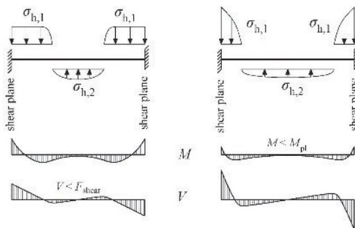
Figure 6: Qualitative distributions for shear force V and bending moment M for high density timber on the left and very high density timber on the right.
