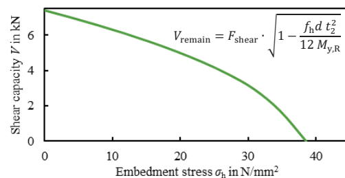
Figure 5: Decrease of remaining shear capacity V_{\text{remain}} with higher embedment stress for a connection with aluminium dowel and 30 mm timber thickness. Uniform embedment stress distribution assumed.
