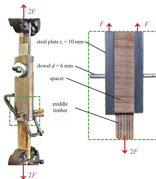
Figure 1: Test setup for connection tests.
