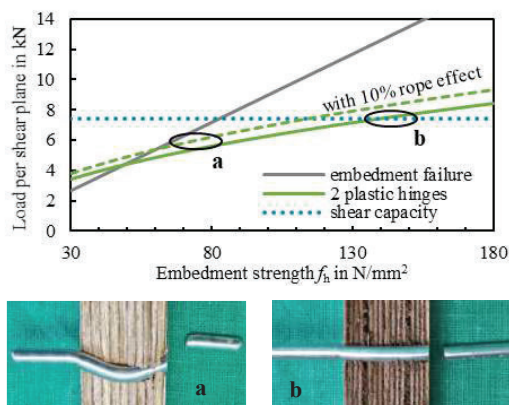
Figure 4: Visualised dependency of different failure modes for aluminium dowels with 30 mm timber thickness.
