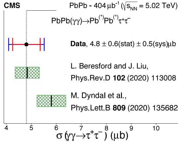
Fig. 109. The \sigma(\gamma\gamma \rightarrow \tau^+\tau^-) cross section, measured in a fiducial phase space region at \sqrt{s_{NN}} = 5.02 TeV. The theoretical predictions [581,582] are computed with leading order accuracy in QED and are represented by the vertical solid lines, which can be compared with the vertical dotted line representing this measurement. The outer blue (inner red) error bars represent the total (statistical) uncertainties, whereas the green hatched bands correspond to the uncertainty in the theoretical predictions, as described in the text. The potential electromagnetic excitation of the outgoing Pb ions is denoted by (*).
