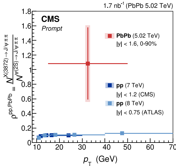
Fig. 79. The yield ratio \rho_{pp,PbPb} of prompt X(3872) over \psi(2S) production in pp and PbPb collisions as a function of p_T . Source: Figure adapted from Ref. [431].
