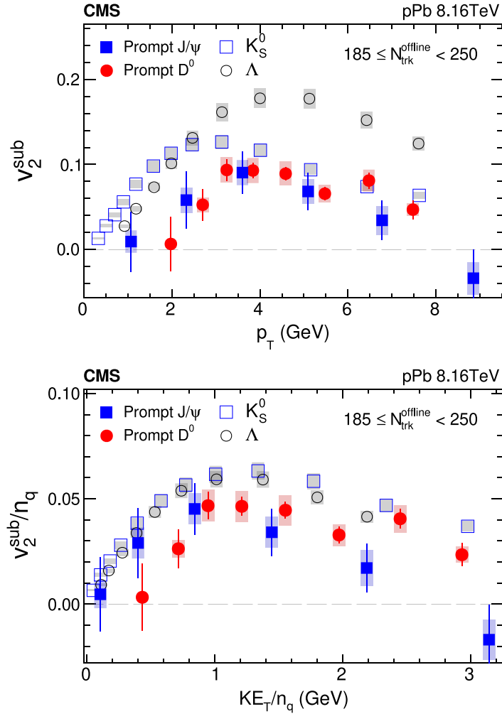
Fig. 92. Upper: The v_2^{\text{sub}} values for prompt J/\psi mesons at forward rapidities ( -2.86 < y_{\text{cm}} < -1.86 or 0.94 < y_{\text{cm}} < 1.94 ), as well as for K_S^0 and \Lambda hadrons, and prompt D^0 mesons at midrapidity ( -1.46 < y_{\text{cm}} < 0.54 ), as a function of p_T for pPb collisions at \sqrt{s_{\text{NN}}} = 8.16 TeV with 185 \leq N_{\text{trk}}^{\text{offline}} < 250 . Lower: The n_q -normalized v_2^{\text{sub}} results. The vertical bars correspond to statistical uncertainties, while the shaded boxes denote the systematic uncertainties. Source: Figure adapted from Ref. [524].
