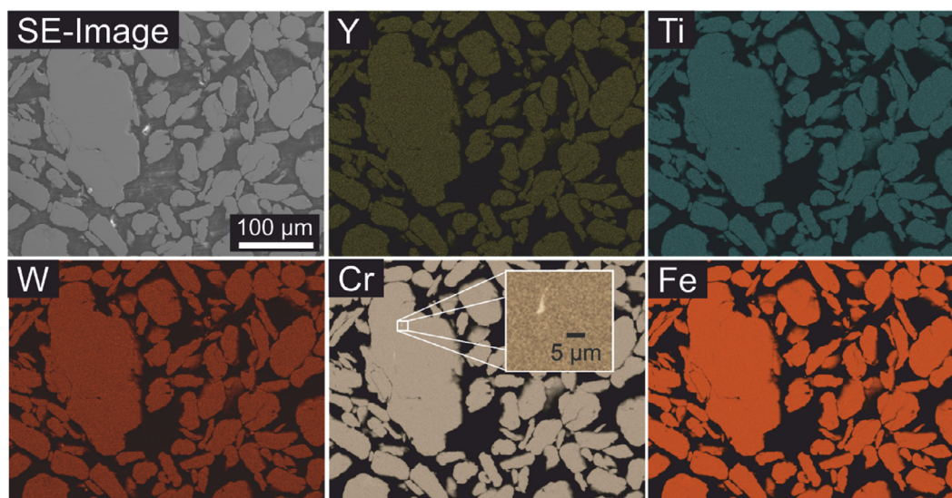
Fig. 1. SEM images of PCA-1 powder after 40 h of mechanical alloying. The magnified area shows an enrichment of chromium with a size of 6 µm.
