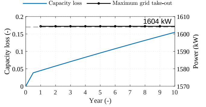
Fig. 9. Ten-year simulation with battery life assessment.
