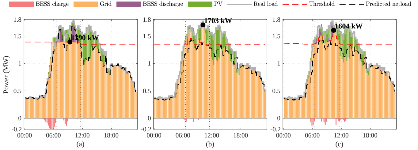
Fig. 5. Power distribution for 3 scenarios on the observation day with maximum netload of 1703 kW. The red dashed line is the optimized threshold \theta^{\text{init}} + \gamma_t . (a) Benchmark: 2 successes out of 2 attempts, with the maximum realized grid power reaching 1390 kW between 06 : 30 and 11 : 30. (b) MPC: 0 success out of 2 attempts, with the maximum realized grid power of 1703 kW at 10 : 15. (c) SMPC: 2 successes out of 6 attempts, with the maximum realized grid power reaching 1604 kW at 10 : 30.
