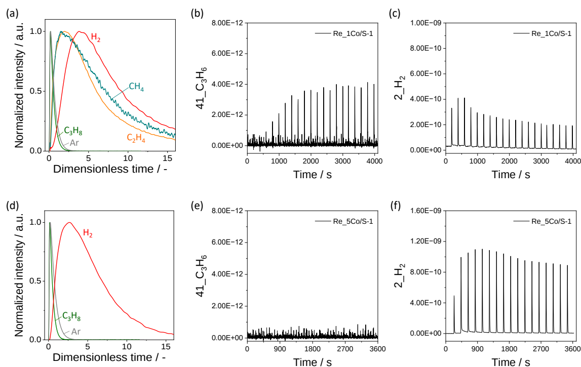
Figure 7. The normalized transient responses recorded upon pulsing of a C_3H_8:Ar = 1:1 mixture at 550^\circ C over reduced (a) 1Co/S-1 and (d) 5Co/S-1 . (b,e) C_3H_6 and (c,f) H_2 response recorded at 550^\circ C after pulsing (1mL) of an C_3H_8/Ar=1:19 mixture over reduced (b,c) 1Co/S-1 and (e,f) 5Co/S-1 . Before the C_3H_8 pulses, the catalysts were exposed to a flow of H_2/Ar=1:4 (10 mL/min) at 550^\circ C for 30 min and then flushed with Ar for 20 min.
