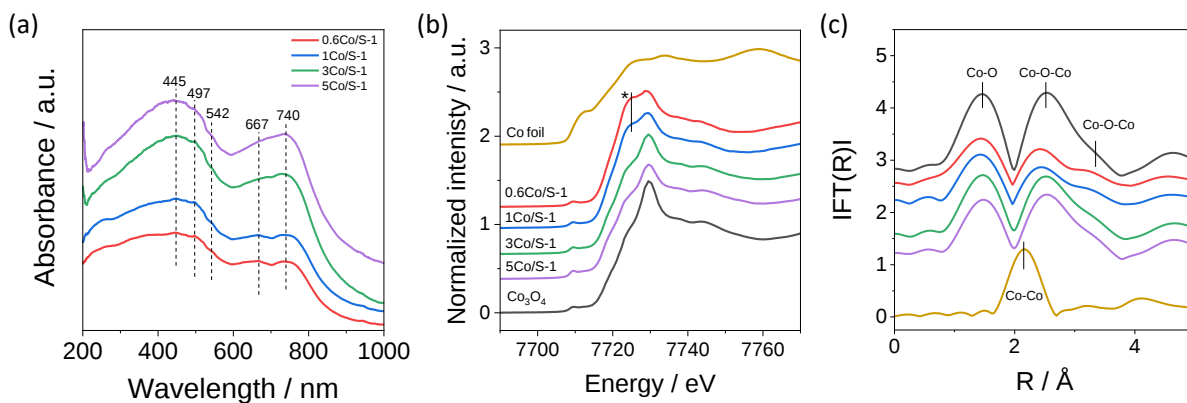
Figure 2. (a) UV-Vis spectra and (b) Co K-edge XANES of the fresh catalysts and reference samples ( \text{Co}_3\text{O}_4 and Co foil). The corresponding k^2 -weighted Fourier transform spectra are shown in (c).
