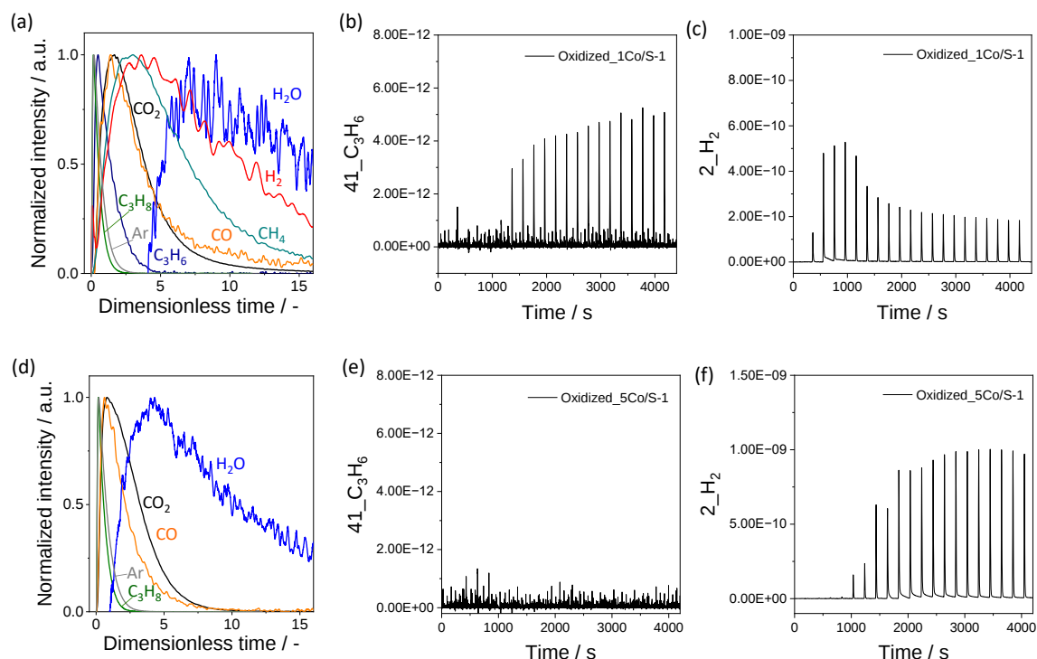
Figure 6. The normalized transient responses recorded upon pulsing a C_3H_8:Ar = 1:1 mixture at 550^\circ C over oxidized (a) 1Co/S-1 and (d) 5Co/S-1. (b,e) C_3H_6 and (c,f) H_2 response recorded at 550^\circ C after pulsing (1mL) of a C_3H_8/Ar=1:19 mixture over oxidized (b,c) 1Co/S-1 and (e,f) 5Co/S-1. Before the C_3H_8 pulses, the catalysts were exposed to a flow of O_2/Ar=1:4 (10 mL/min) at 550^\circ C for 30 min and then flushed with Ar for 20 min.
