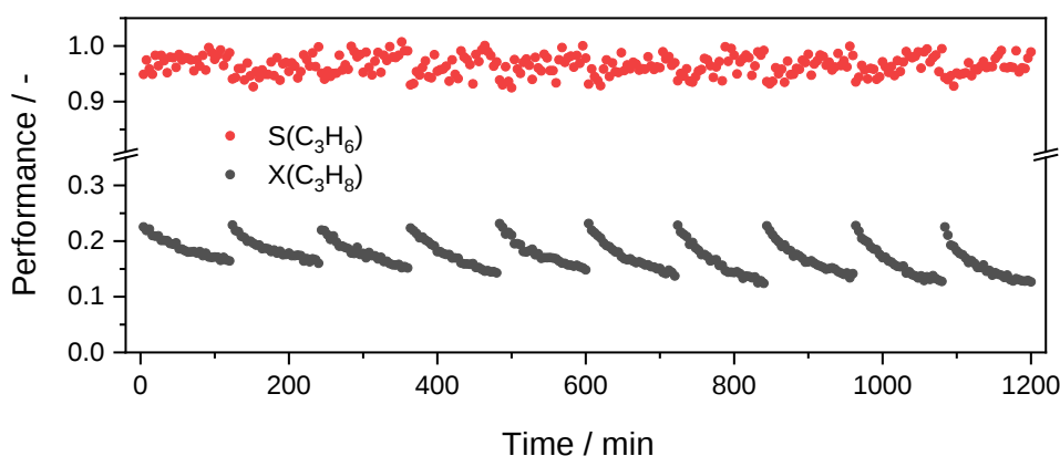
Figure 10. Propane conversion and propene selectivity over 1Co/S-1 in 10 PDH/ regeneration cycles. Reaction conditions: T=550^\circ\text{C} , catalyst amount=100mg, WHSV(C_3H_8)=4.7 \text{ h}^{-1} , C_3H_8:N_2=2:3 . Each cycle consisted of a PDH stage lasted for 120 min and a regeneration stage lasted for 30 min.
