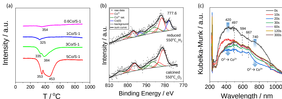
Figure 3. (a) H 2 -TPR profiles of xCo/S-1. (b) Quasi in situ XP spectra of 1Co/S-1 after treatment at 550°C with 20vol% O 2 /Ar or 40vol% H 2 /Ar. (c) In situ UV-Vis spectra of 1Co/S-1 after treatment at 550°C with 40vol% H 2 /Ar.
