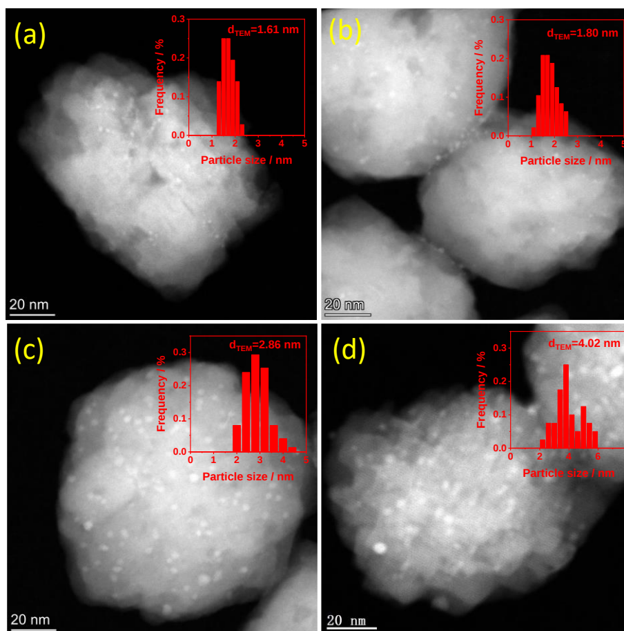
Figure 1. HAADF-STEM images of as-prepared (a) 0.6Co/S-1, (b) 1Co/S-1, (c) 3Co/S-1 and (d) 5Co/S-1.
