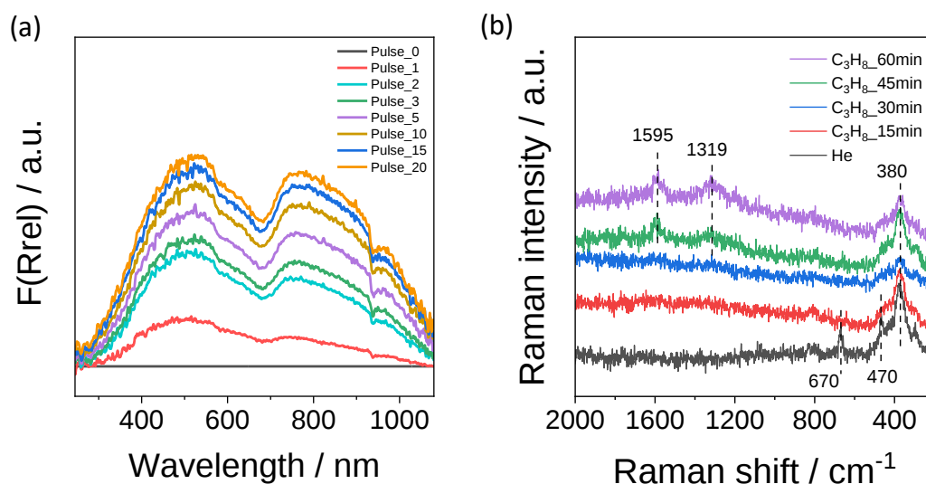
Figure 8. (a) Operando UV–Vis spectra of 1Co/S-1 during the C 3 H 8 pulses (1mL pulse size) at 550°C using a feed with 5vol% C 3 H 8 in Ar. (b) Operando Raman spectra of 1Co/S-1 collected during exposure to a feed with 40vol% C 3 H 8 in N 2 at 550°C.
