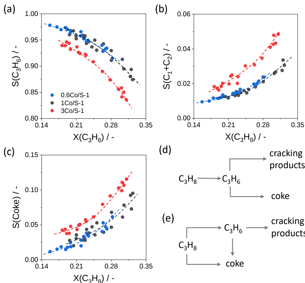
Figure 5. The selectivity-conversion relationships for (a) propene, (b) \text{C}_1 - \text{C}_2 hydrocarbons and (c) coke formed over 0.6Co/S-1, 1Co/S-1 and 3Co/S-1. Proposed reaction pathways for propane dehydrogenation over (d) 0.6Co/S-1 and 1Co/S-1 as well as (e) 3Co/S-1. Reaction conditions: T=550^\circ\text{C} , \text{C}_3\text{H}_8:\text{N}_2=2:3 , \text{WHSV}(\text{C}_3\text{H}_8)=2.4\text{--}14.1\text{ h}^{-1} .
