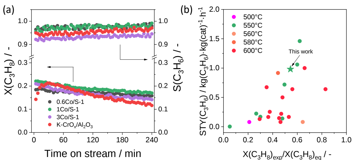
Figure 9. (a) Time-on-stream profiles of propane conversion and propene selectivity over tested samples. (b) Space time yield of propene formation ( \text{STY}(\text{C}_3\text{H}_6) ) determined over 1Co/S-1 and previously reported Co-based catalysts (Table S4) versus X(\text{C}_3\text{H}_8)_{\text{exp}}/X(\text{C}_3\text{H}_8)_{\text{eq}} . Reaction conditions: T=550^\circ\text{C} , catalyst amount=100mg, \text{WHSV}(\text{C}_3\text{H}_8)=4.7 \text{ h}^{-1} , \text{C}_3\text{H}_8:\text{N}_2=2:3 .
