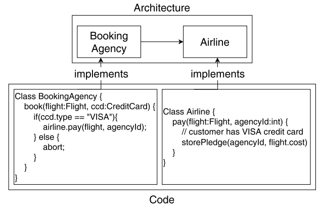
Figure 8: The Architecture contains the Booking Agency and the Airline with their data flows. The Code contains possible implementations violating the security specifications by allowing the information about the type of the credit card to flow to the Airline . This may be because the Booking Agency has a new collaboration with VISA as an evolved system requirement.
