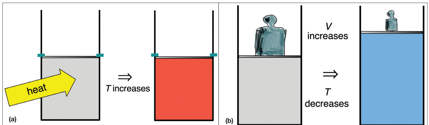
Fig. 1. (a) The temperature increases when heat is supplied; (b) it decreases when the volume is increased.
