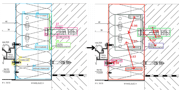
Figure 4. Ground truth correspondences (left) and predicted correspondences (right) for a successful example (cropped). The predicted correspondences match the ground truth exactly, demonstrating the model's reliability when trained with sufficient plans with a similar visual appearance.
