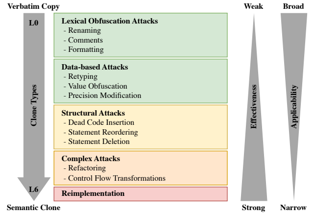
Fig. 1: Categorization of obfuscation attacks according to Karnalim [10] and Faidhi and Robinson [33], illustrating obfuscation effectiveness and applicability.
