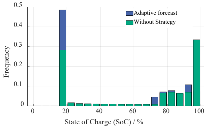
Figure 6. Impact of adaptive forecast on SoC distribution
