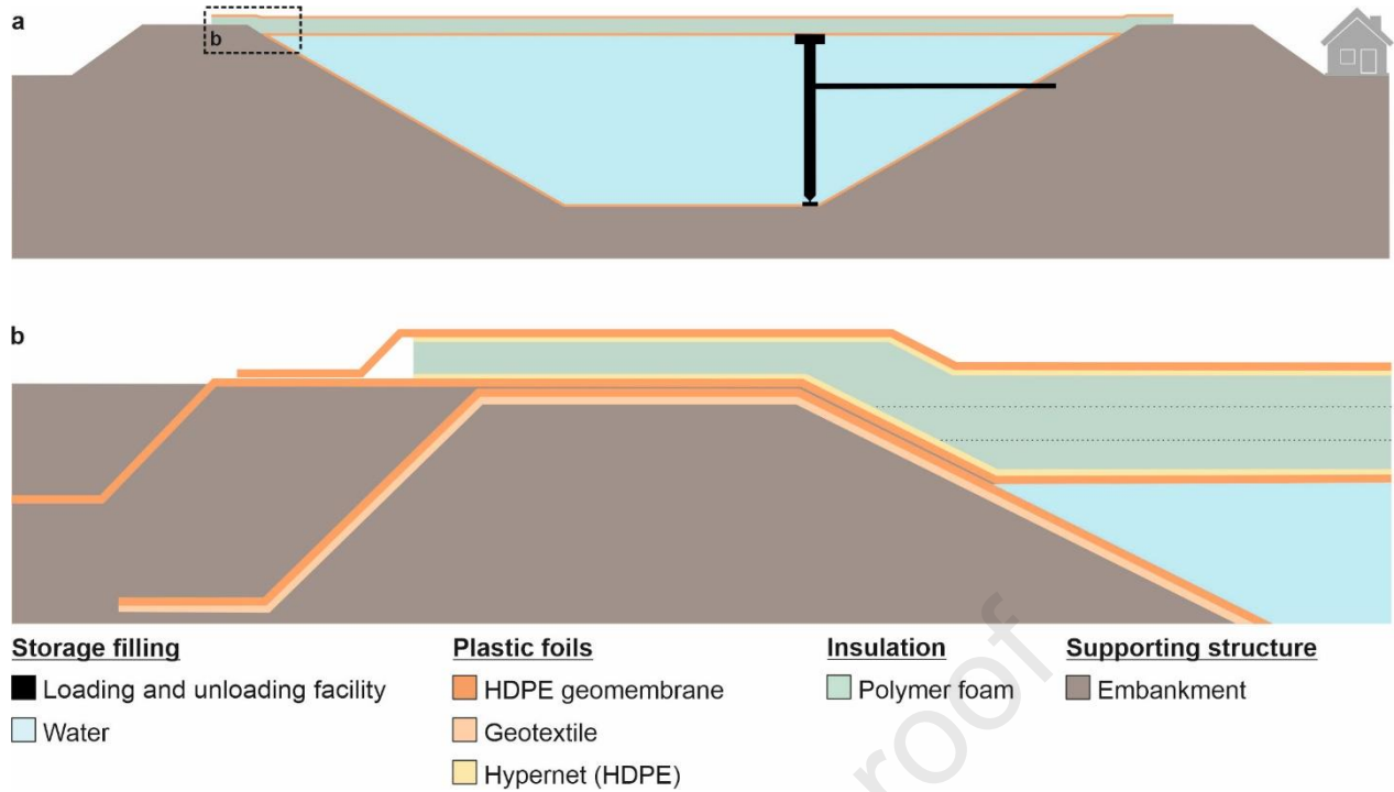
Fig. 2 a. Schematic layout of the pit thermal energy storage (PTES) based on Marstal in relation to a typical single-family house for a general size indication (not to scale); b. detailed section of the PTES, highlighting the specific materials used, based on [31,52,53,57]. HDPE: High-density polyethylene.
