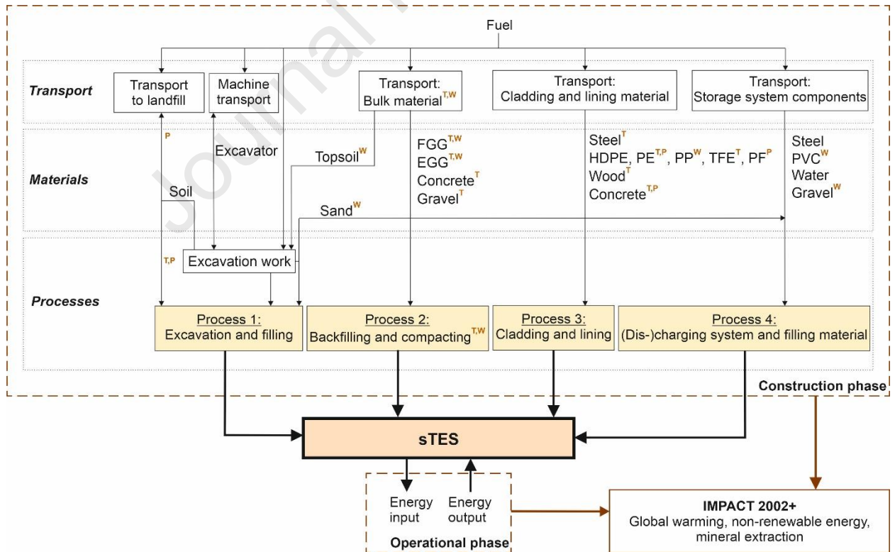
Fig. 4. Process visualization of the three selected sTES prototypes, according to [41]. T: Processes only applicable to TTES; P: Processes only relevant to PTES; W: Processes only relevant to WGTES. FGG: foam glass gravel, PP: polypropylene, PF: polymer foam, PE: polyethylene, HDPE: high-density polyethylene, EGG: expanded glass granulate, TFE: tetrafluoroethylene, PVC: polyvinyl chloride.
