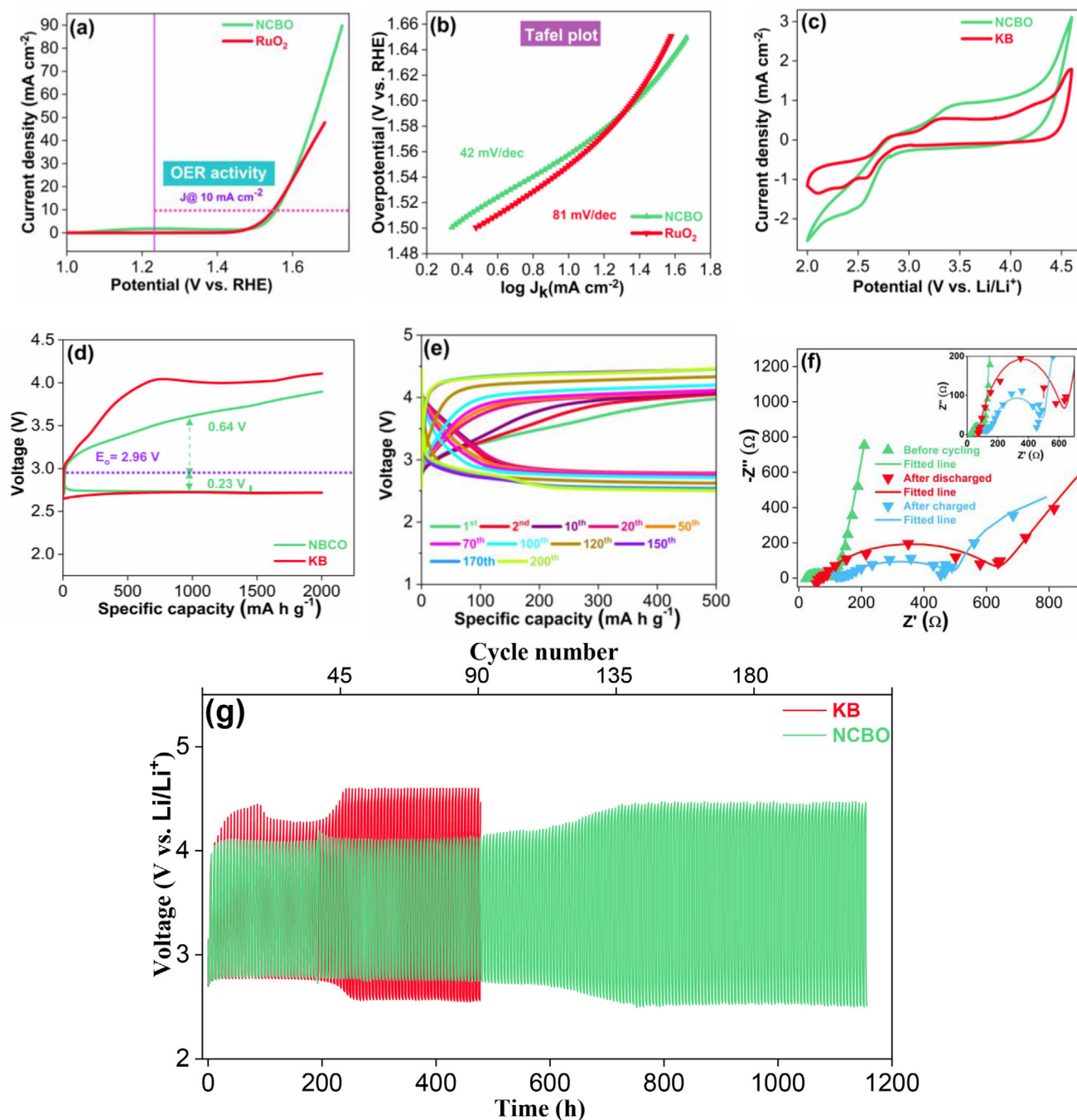
Figure 3. a) iR-corrected LSV plots of OER and b) Tafel plots of the NCBO and \text{RuO}_2 catalysts in 1 M KOH electrolyte. c) CV curves of NCBO and KB electrodes at a scan rate of 0.1 \text{ mV s}^{-1} and between 2.0 and 4.5 V. d) The discharge/charge profiles of the NCBO and KB electrodes at a current density of 175 \text{ mA g}^{-1} and a cut-off capacity of 2000 \text{ mA h g}^{-1} . e) Cyclic stability test of the NCBO \text{O}_2 cathode (current density of 175 \text{ mA g}^{-1} , cut-off capacity of 500 \text{ mA h g}^{-1} ). f) Nyquist plots (inset: higher magnification of Nyquist plots) and g) long cycle stability test for NCBO and KB electrodes at a current density of 175 \text{ mA g}^{-1} .
