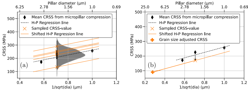
Fig. 3. Graphic description of the grain size scaling algorithm based on the Hall–Petch-relation. (a) Schematic depiction of the shifting of the Hall–Petch regression lines based on the 2 \mu\text{m} pillar CRSS-distribution, (b) Schematic depiction of the calculation of the grain size adjusted \xi_0 material parameter (cf. alg. 1).
