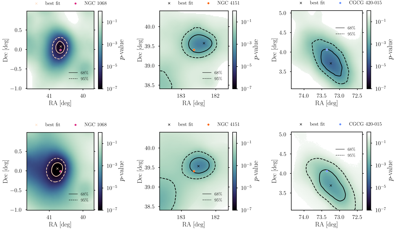
Figure 2. Local (pretrial) p -value maps around the most significant sources NGC 1068 (left), NGC 4151 (middle), and CGCG 420-015 (right) with the disk-corona model fit (top) and the power-law fit (bottom). Colored points show the locations of sources and crosses show the best-fit locations. Contours correspond to 68% (solid) and 95% (dashed) confidence regions.
