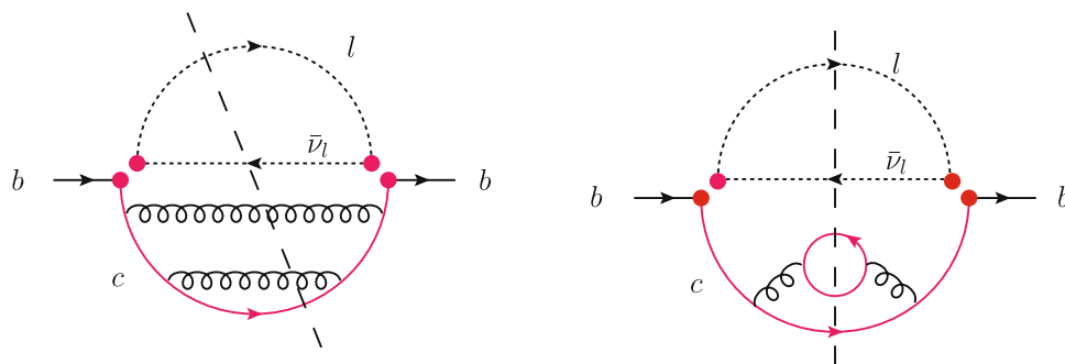
Fig. 21 Sample diagrams whose imaginary part contributes to the semileptonic B meson decays at NNLO. The dashed lines represent the charged lepton neutrino pair. Black solid lines denote bottom quarks, magenta lines denote charm quarks, respectively
