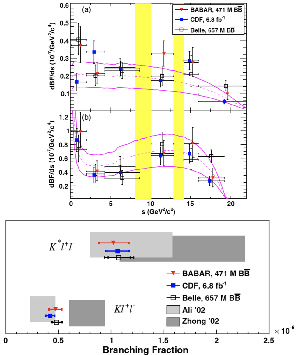
Fig. 10 (Up): Partial branching fractions for the a B \rightarrow K\ell^+\ell^- and b B \rightarrow K^*\ell^+\ell^- as function of s showing BABAR measurements (red triangle) and the SM prediction from the Ali et al. model [119]. (Down): Total branching fraction for the B \rightarrow K\ell^+\ell^- and B \rightarrow K^*\ell^+\ell^- from Babar (red triangle), compared with Belle (open squares) [123] and CDF (blue solid) [125] measurements and with predictions of Ali et al. model [119] and Zhong, Wu and Wang [128]. (From Lees et al. (BABAR collaboration) Phys Rev. D86, 032012 (2012))
