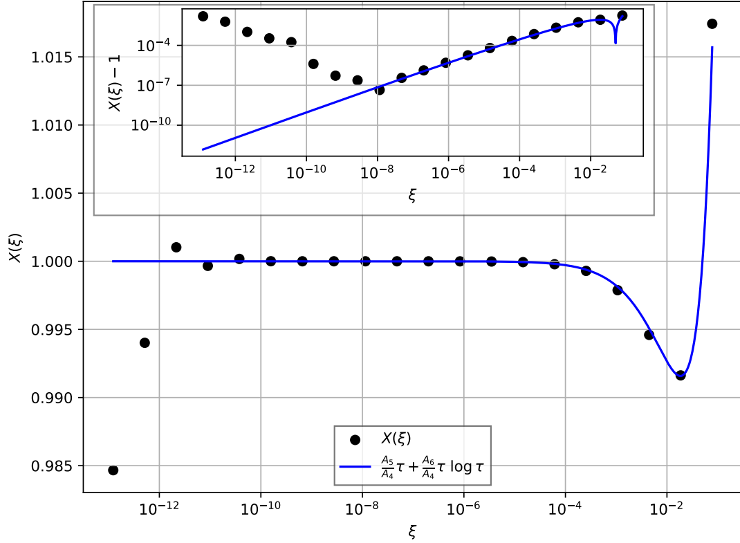
Figure 1. The parameter X(\tau) expressed as a function of \xi , which relates the small-jettiness expansions of the vector boson production cross section and a numerical integration of (2.16) at Q = 100 GeV and m_V = 90 GeV and with the Gaussian luminosity distribution given in eq. (2.36). The parameter approaches unity for lower values of \xi before the numerical integration becomes unreliable. A fit of the missing linear terms in \tau is presented in blue.
