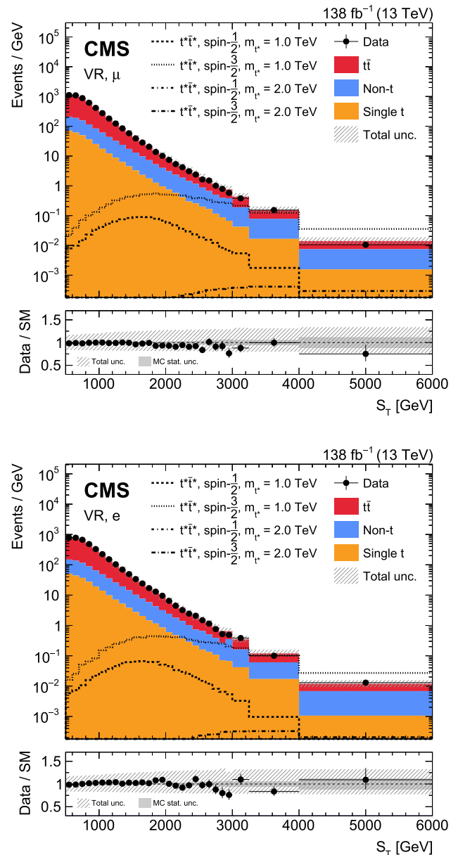
Fig. 5 Distributions of S_T in the VR for the muon (upper) and electron (lower) channels. The total uncertainties are shown as hatched bands. The signal distributions are scaled to the cross sections predicted by theory. Ratios of data to the expected backgrounds are shown in the lower panels
