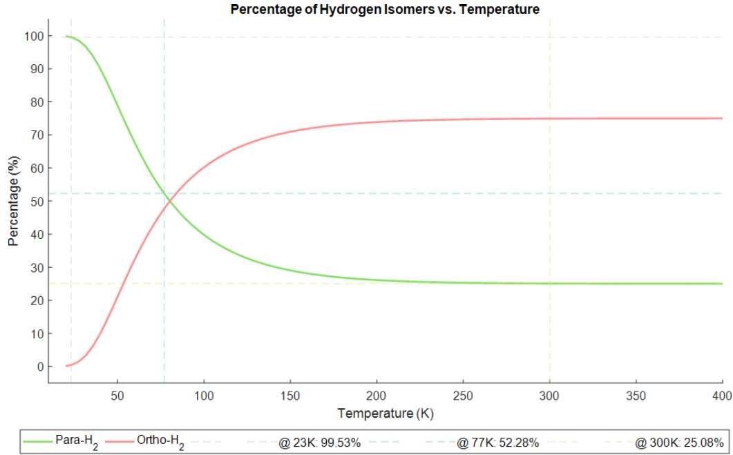
Figure 3.2: Equilibrium percentage of para -H 2 as a function of temperature. More details of the calculation in MATLAB can be found in Appendix A.1.
