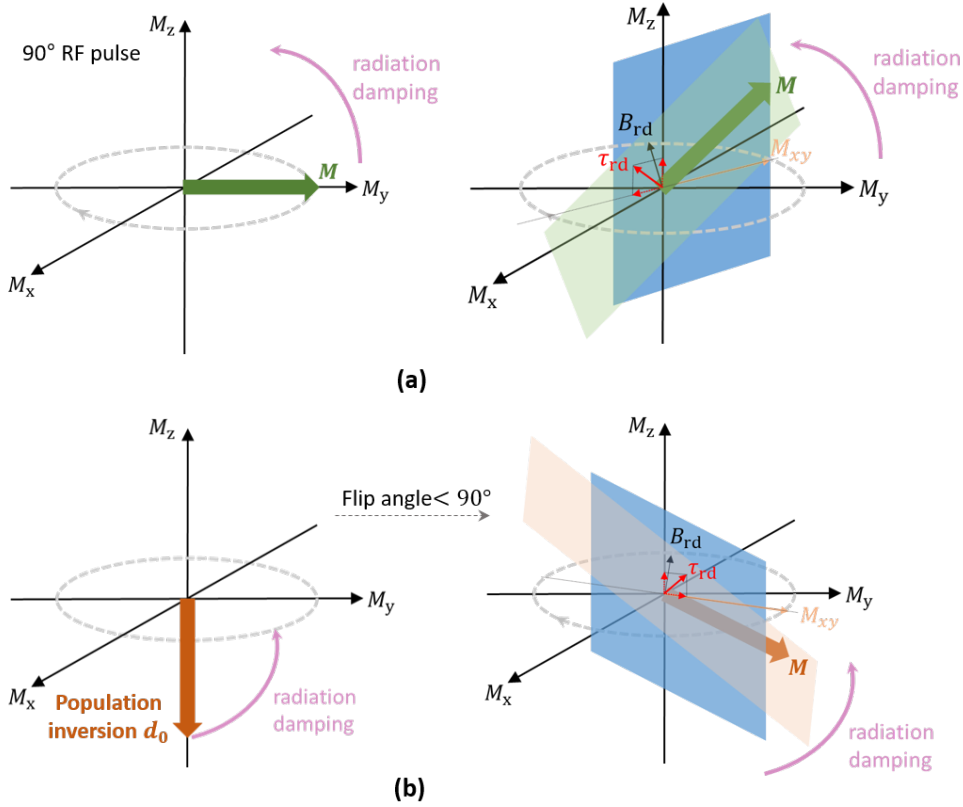
Figure 6.1: Schematic showing the effect of radiation damping ( \tau_{rd} ) in the case of (a) normal NMR detection with a 90° RF pulse applied on a positive magnetization and (b) negative longitudinal magnetization with a small flip-angle.
