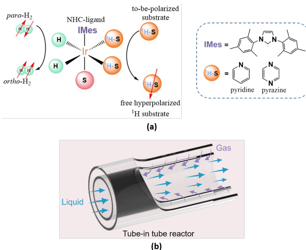
Figure 5.1: (a) Schematic representation of SABRE hyperpolarization on a catalytic complex. The spin orders derived from para -H 2 are transferred to the substrates (pyridine and pyrazine) on the equatorial plane through the J-coupling network. The hyperpolarized substrates with boosted magnetization dissociate from the catalyst form free substrates without chemical modification. (b) Section view of the tube-in-tube reactor under countercurrent condition.
