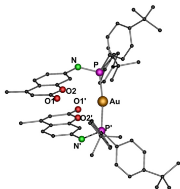
Fig. 2 Molecular structure of the cationic part of gold(I) complex 2 in the solid state. Hydrogen atoms, non-coordinating solvents and the SbF 6 − anion are removed for clarity. Selected bond distances (Å) and angles (°): Au–P 2.305(2), N–P 1.676(5); P–Au–P 171.63(8). 48
