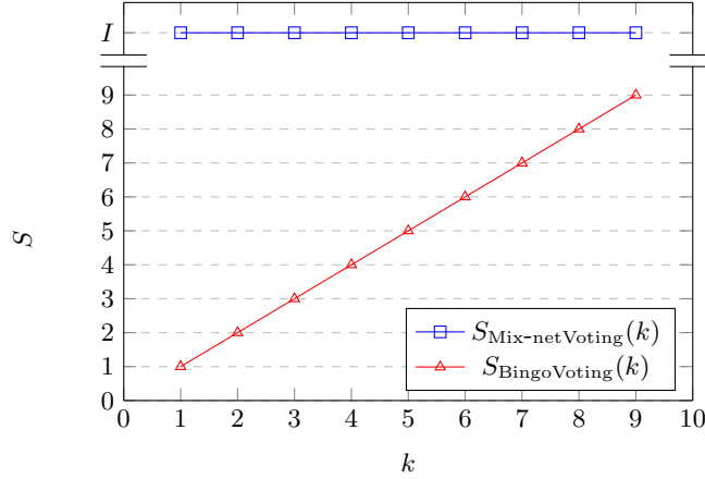
Figure 2. Scalability of attacks on voting schemes. For Mix-net Voting, the scalability of the attack on the confidentiality is displayed, which is also the overall (maximum) scalability of the scheme. For Bingo Voting, the scalability of attacks on the confidentiality and integrity coincide.
