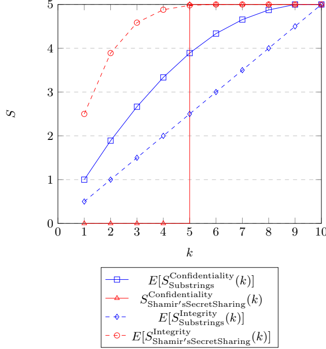
Figure 3. Scalability of attacks on secret sharing schemes when using ten servers. Attacks on confidentiality as well as integrity are considered. For the substring approach and the integrity of Shamir's secret sharing scheme, expected values are displayed.
