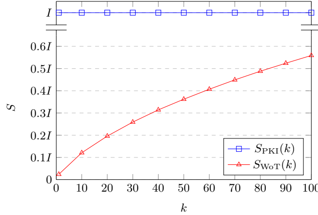
Figure 1. Scalability of attacks on authentication infrastructures. The scaling curves for attacks on the confidentiality and integrity coincide for both the PKI and the WoT.
