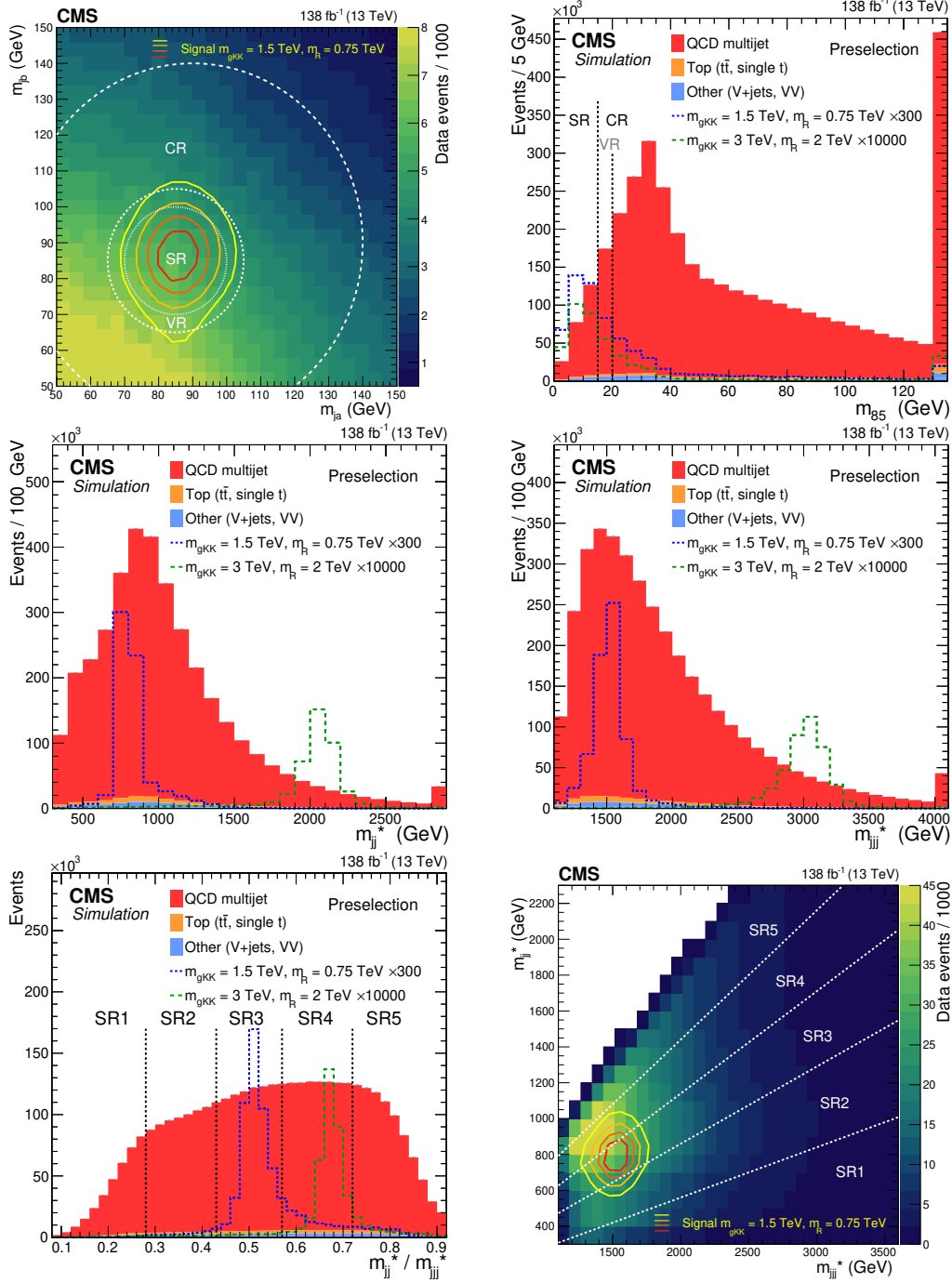
Figure 3. Distributions after event preselection. Upper left: the two-dimensional ( m_{ja}, m_{jb} ) distribution for a posited signal ( m_R = 0.75 \text{ TeV} , m_{g_{KK}} = 1.5 \text{ TeV} ) compared to the background-dominated data. For signal, contours corresponding to 80, 60, 40, and 20% of the maximum signal event yield are shown for shape visualization. White dashed curves indicate boundaries between SR, VR (defined in section 6.1), and CR areas. The one-dimensional histograms show the m_{85} (upper right), m_{jj}^* (middle left), m_{jjj}^* (middle right), and m_{jj}^*/m_{jjj}^* (lower left) distributions using simulated signal and background events, as indicated in the legends. The signal events are scaled by the labeled factors times the theoretical cross sections for visibility. Lower right: the two-dimensional ( m_{jj}^*, m_{jjj}^* ) distribution in data. White dashed lines indicate the SR splitting.
