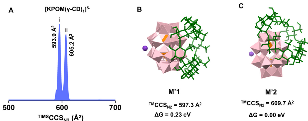
Fig. 5 (A) TMS spectra of [KPOM(\gamma\text{-CD})_1]^{5-} , (B and C) DFT-optimized lowest energy structures of [KPOM(\gamma\text{-CD})_1]^{5-} . ^{TMS}CCS_{N_2} values denote the mean values over three measurements. The standard error is \leq 1.0 \text{ \AA}^2 . \Delta G is the relative free energy, computed using the \omega B97X\text{-}V/\text{def}2\text{-}TZVPP method. Color codes: pink: WO_6 octahedron, orange: PO_4 tetrahedron, green: \gamma\text{-CD} .
