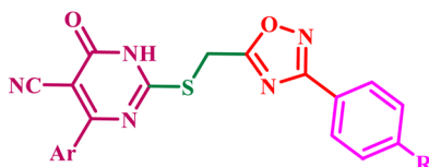
Target compounds (10a-l)
