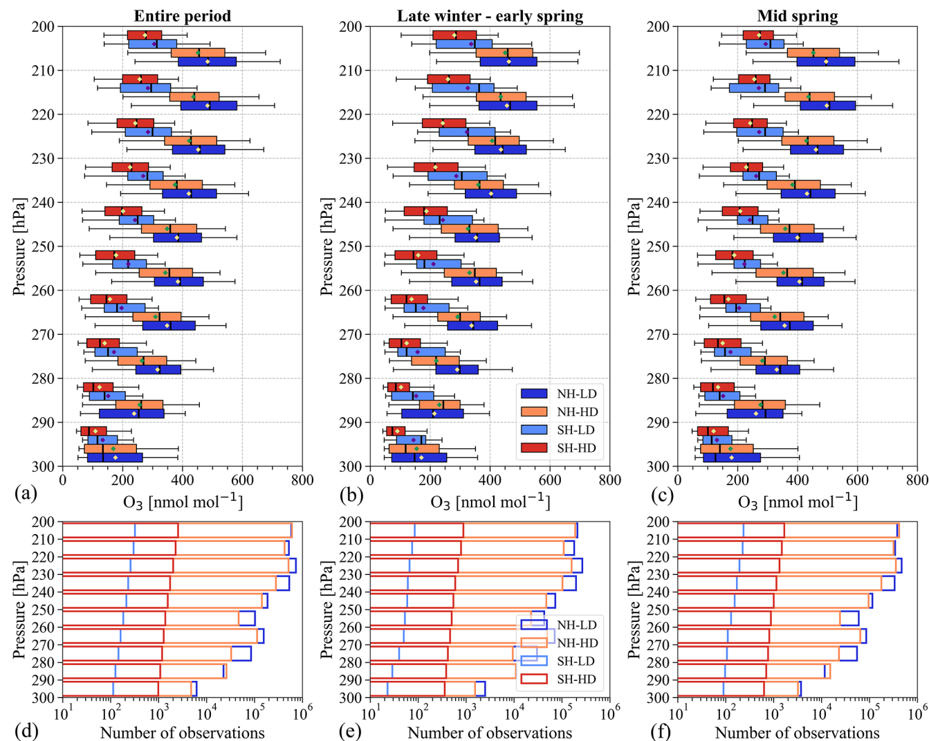
Figure B1. Ozone boxplot (nmol mol -1 ) and associated sample sizes by pressure bins. The plots include ozone data with RH less than 20 % obtained exclusively from IAGOS and WUOUC (Table 1). In the upper panel, (a), (b) and (c) show the entire period, late winter–early spring and mid-spring, respectively, for the Northern Hemisphere and Southern Hemisphere and HD and LD years. Boxplots indicate the median and the 25th and 75th percentiles. The diamonds in panels (a)–(c) indicate the mean values. The whiskers extend to the 5th and 95th percentiles. In panels (d)–(f), the x axis shows the observation numbers. The rest of the plot information is the same as described in panels (a)–(c). High- and low-depletion years in SH included ozonesondes launched from Ushuaia, Lauder and Macquarie Island.
