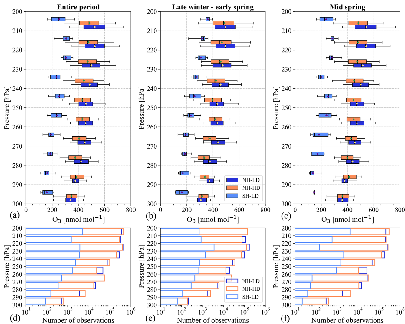
Figure C1. Ozone boxplot ( \text{nmol mol}^{-1} ) and associated observation numbers by pressure bins. The plots include ozone data with CO less than 50 \text{ nmol mol}^{-1} . In the upper panel, (a), (b) and (c) show the entire period, late winter–early spring and mid-spring for the Northern Hemisphere and Southern Hemisphere and HD and LD years. Boxplots indicate the median and the 25th and 75th percentiles. The diamonds in (a)–(c) indicate the mean values. The whiskers extend to the 5th and 95th percentiles. In panels (d)–(f), the x axis shows the observation numbers. The rest of the plot information is the same as described in (a)–(c).
