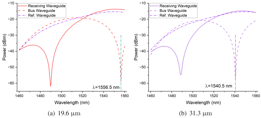
Figure 7.23: Transmission spectra of the fixed directional couplers in TM mode with lengths of (a) 19.6 \mu\text{m} and (b) 31.3 \mu\text{m} .
