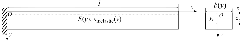
Figure 4.1: Sketch of a general Euler-Bernoulli beam model. Elastic modulus, inelastic strains and width vary in thickness direction. The distance between the top surface of beam and centroid in the cross section is marked as y_c .
