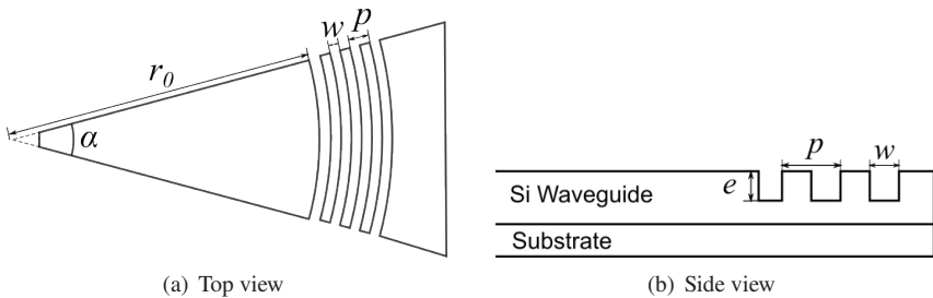
Figure 7.2: (a) Top and (b) side view of the grating coupler with the design parameters.
