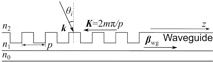
Figure 3.7: Illustrative Bragg condition for periodic grating coupler.
