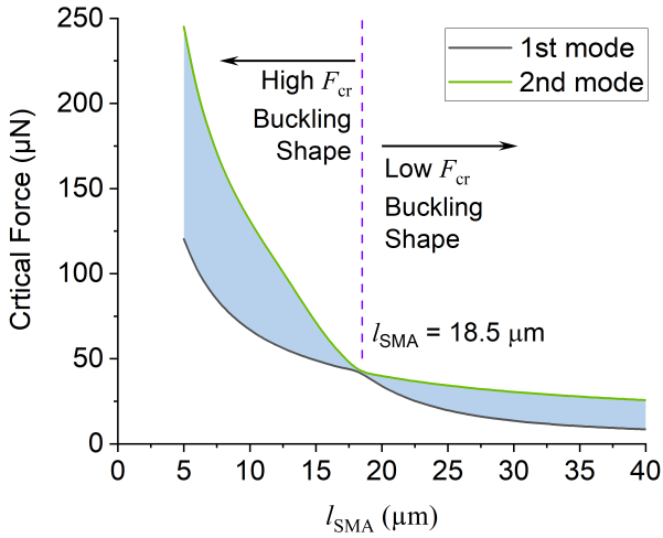
Figure 6.8: Influence of the length of Beam II, l_{\text{SMA}} , on the first- and second-mode critical force of buckling. Shaded area represents the region that the compressive force should fall into to create buckling.
