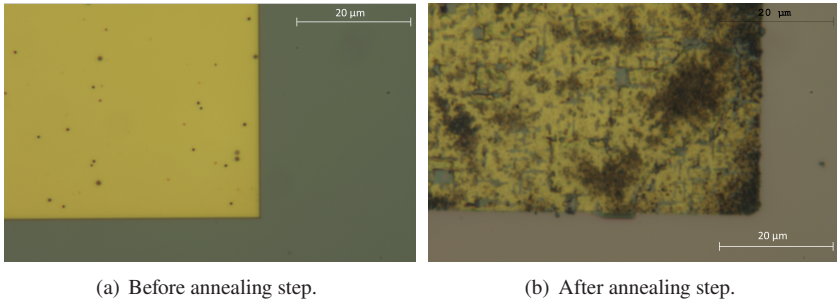
Figure 2.5: Comparison of a corner of the gold marker (a) before and (b) after the annealing step for the SMA layer.
