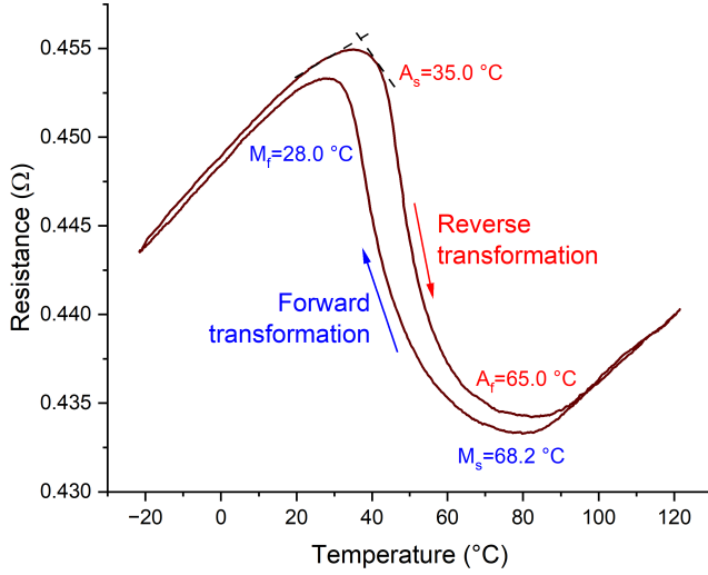
Figure 5.3: Temperature-resistance curve of a sputtered 600 nm-thick \text{Ti}_{54}\text{Ni}_{31}\text{Cu}_{15} film on Si substrate. Transformation temperatures marked in the figure are determined by the tangential method.
