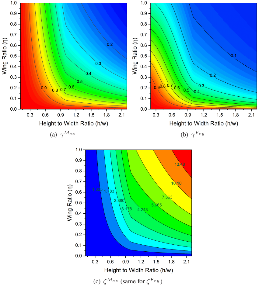
Figure 4.9: Influences of wing ratio \eta and height to width ratio h/w of cross-section on structural stiffness ratio (a) \gamma^{Mez} (b) \gamma^{Fey} and (c) \zeta^{Mez} (same for \zeta^{Fey} ). Calculation based on half of monomorph double-beam structure in Fig. 4.7(b).
