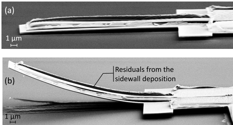
Figure 6.19: SEM images of the structure in Fig. 6.14(a) after depositing the SMA layer (Step (d) of fabrication process), (a) before and (b) after the annealing of SMA layer.
