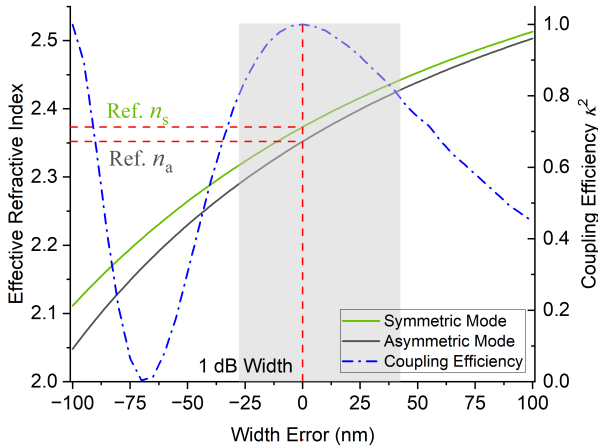
Figure 7.9: Relations of the symmetric and asymmetric refractive indices n_s and n_a , and the coupling efficiency \kappa^2 versus the errors of the waveguide width. The shaded area represents the 1 dB width of the error range.
