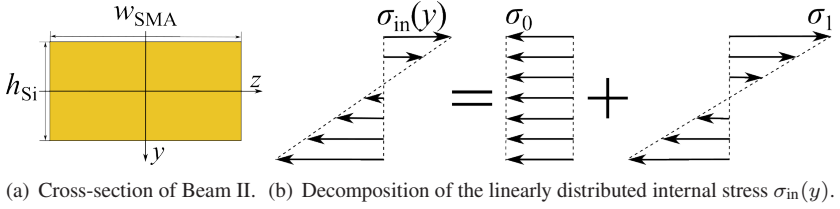
Figure 6.16: (a) The cross-section of Beam II and (b) the linear distribution of the internal stress \sigma_{\text{in}}(y) in the Si layer. \sigma_{\text{in}}(y) is decomposed into a uniform term \sigma_0 and a proportional term.
