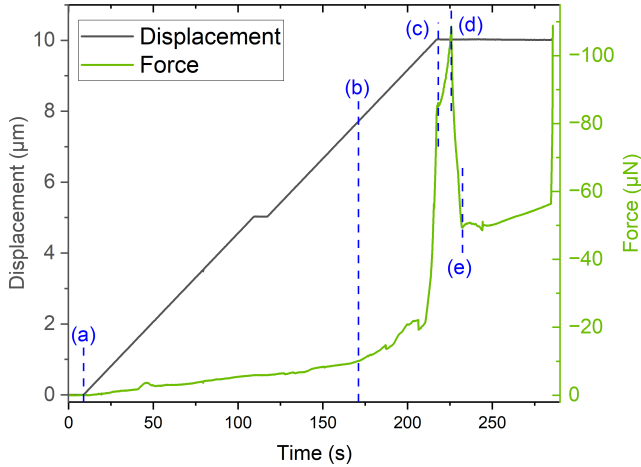
Figure 6.20: Loading curves (Displacement and Force versus Time) of structure with the following dimensions: l_{\text{SMA}} = 40 \mu\text{m} , w_{\text{SMA}} = 2.2 \mu\text{m} , l_{\text{Si}} = 25 \mu\text{m} , w_{\text{Si}} = 1.4 \mu\text{m} . The structural shapes at Point (a)–(e) are shown in Fig. 6.21. The minus force represents the direction.
