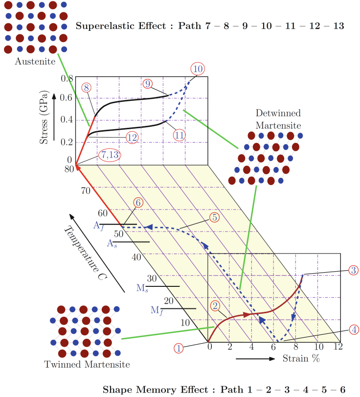
Figure 2.2: A three-dimensional strain-stress-temperature graph illustrating both the shape memory effect (path 1–6) and the pseudoelastic effect (path 7–13) of SMAs. Picture adapted with permission from [2].
