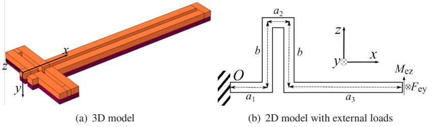
Figure 4.7: (a) 3D and (b) 2D model of a multilayer double-beam cantilever with wing structure design. Due to symmetry, only half of the structure is considered. The structural dimensions and external loads are marked out.
