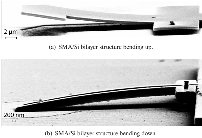
Figure 5.11: SMA/Si bilayer structures on the same chip show different bending directions: (a) bending-up, (b) bending-down.
