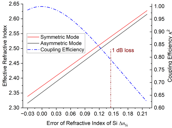
Figure 7.13: Relations of the symmetric and asymmetric refractive indices n_s and n_a , and the coupling efficiency \kappa^2 versus the error of the refractive index of Si \Delta n_{\text{Si}} . In the studied error range, the loss is above 1 dB when \Delta n_{\text{Si}} > 0.144 .
