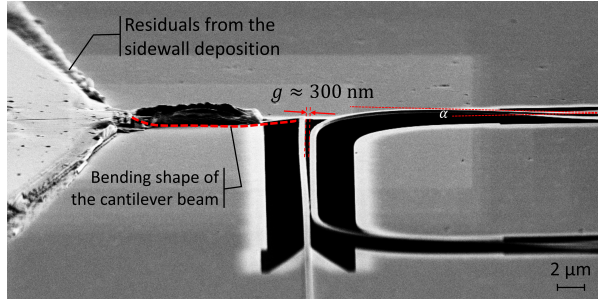
(a) Side view of Structure A.
