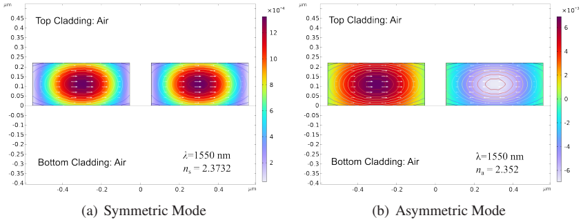
Figure 7.5: (a) Symmetric and (b) asymmetric TE-modes of the directional coupler composed by two strip waveguides with a gap of 110 nm. Both top and bottom claddings are air. The structure is simulated at the wavelength of 1550 nm.
