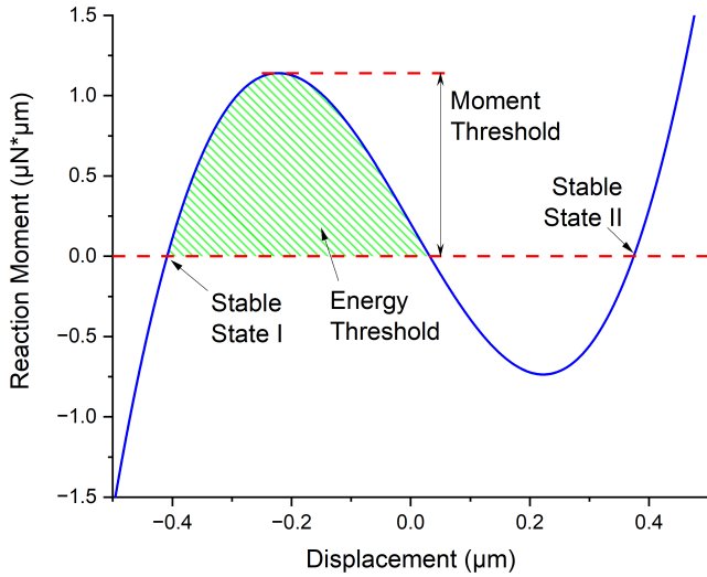
Figure 6.6: Simulated reaction moment-displacement curve of buckled Beam I showing bistability. Parameters used for simulation are listed in Table 6.1. Shaded area represents the energy threshold that needs to be overcome for state-switching.
