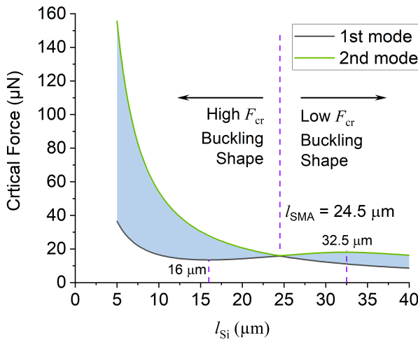
Figure 6.9: Influence of the length of Beam I, l_{Si} , on the first- and second-mode critical force of buckling. Shaded area represents the region that the compressive force should fall into to create buckling.
