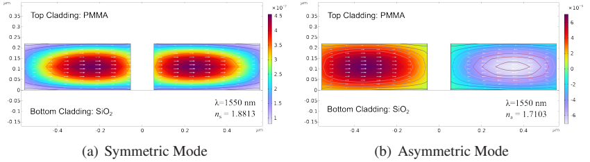
Figure 7.22: (a) Symmetric and (b) asymmetric TM-modes of the directional coupler composed by two strip waveguides with a gap of 110 nm at the wavelength of 1550 nm. The top and bottom claddings are PMMA and SiO 2 , respectively.
