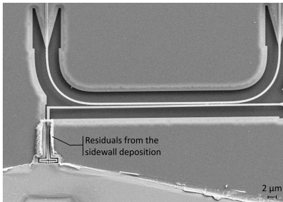
(c) Top view of Structure A.
