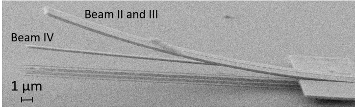
Figure 6.15: After breaking the front connecting the four beams of the structure in Fig. 6.14(a), Beam II and Beam III are still bent up whereas Beam IV becomes flat (Beam I is broken and flies out of the scope of the view).
