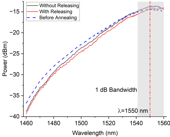
Figure 7.19: Transmission spectra (solid lines) of the reference waveguides with and without partially releasing section after being annealed. The dashed line is from the reference rib waveguide before annealing. The shaded area represents the 1 dB bandwidth of the grating coupler.
