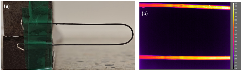
Figure 4.5: Experimental validation of the thermal model by a Joule-heated double-beam cantilever. (a) A tin wire is folded into the shape of a double-beam cantilever structure. Its left ends are connected to the steel pads as the heat sink. (b) The wire is Joule-heated and the temperature distribution is captured by the infrared camera.
