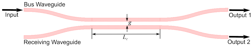
Figure 3.6: Sketch of a directional coupler.
