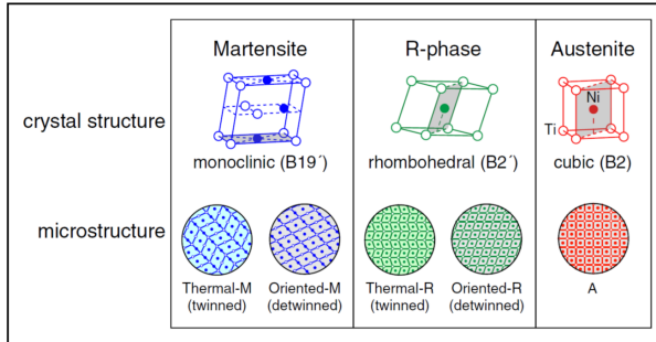
Figure 2.1: Schematics of the crystal structure and microstructure of Ni-Ti alloy at different phases. Diagram adapted with permission from [76].
