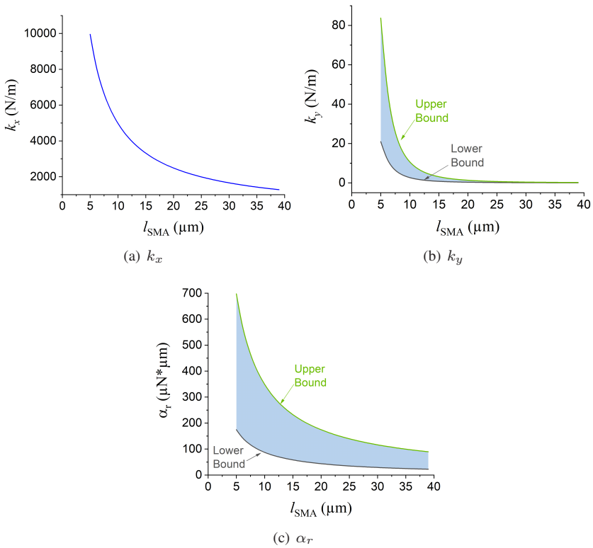
Figure 6.7: Influence of the length of Beam II l_{\text{SMA}} on the spring stiffnesses (a) k_x , (b) k_y and (c) \alpha_r . The shaded areas in (b) and (c) define the regions that the actual spring stiffnesses should fall into.
