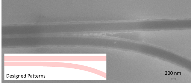
Figure 2.4: An example showing the proximity effect. In the SEM image, the gap between the two waveguides is filled with the residuals of the negative resist. The bottom-left corner shows the designed patterns from the layout file.
