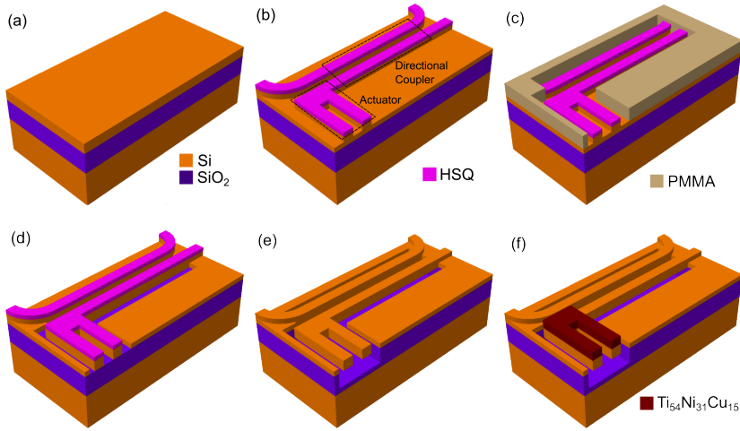
Figure 7.14: Fabrication processes of SMA-based nanoactuator integrated with the directional coupler. (a) The SOI wafer used for fabrication; (b) The shallow Si RIE of 70 nm. The patterns for this etching step are defined by the first EBL exposure with the resist HSQ. (c) A window for the deep Si RIE is defined by the second EBL exposure with the resist PMMA. (d) Deep Si RIE to expose the box layer in the regions that the structures will be released. (e) Wet-etching of SiO 2 to release the free-standing nanoactuators and directional couplers. (f) 300 nm-thick Ti 54 Ni 31 Cu 15 layer is added to the top of the nanoactuators and the electric circuit (not displayed in the figure) by lift-off. The whole wafer is annealed lastly.
