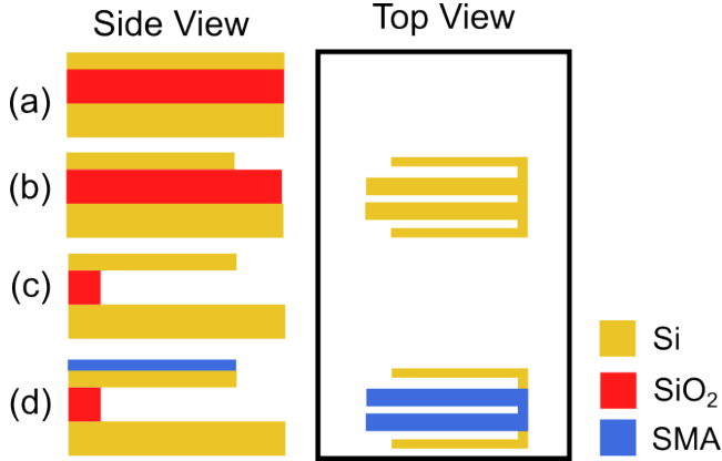
Figure 6.13: Fabrication processes of the SMA nanoactuator with out-of-plane bistability. Starting with (a) the SOI chip, the patterns of nanoactuators and conductive lines are defined by EBL and transferred to the device layer by RIE in step (b). Afterwards, the structures are released by a wet-etching step (c). Lastly, the SMA layer is locally deposited on the two middle beams by lift-off process and annealed in step (d).
