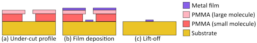
Figure 2.7: Process flow of lift-off process.
