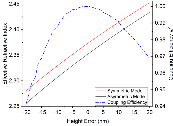
Figure 7.10: Relations of the symmetric and asymmetric refractive indices n_s and n_a , and the coupling efficiency \kappa^2 versus the errors of the waveguide height.
