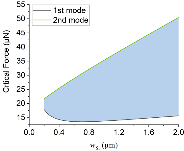
Figure 6.10: Influence of the width of Beam I, w_{Si} , on the first- and second-mode critical force of buckling. The shaded area represents the region that the compressive force should fall into to create buckling.
