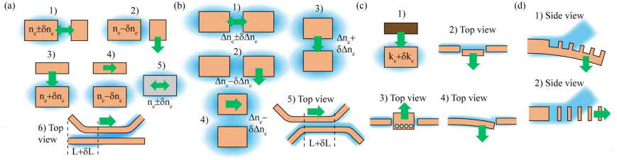
Figure 1.1: Schematics of several MEMS tuning mechanisms. (a) Phase shifting by varying the effective refractive index with loading 1) in-plane, 2) out-of-plane, 3) double-layer out-of-plane, 4) double-layer in-plane, 5) strain tuning, 6) waveguide elongation. (b) Power splitting by variations 1) in-plane, 2) out-of-plane, 3) double-layer out-of-plane, 4) double-layer in-plane, 5) in longitudinal direction. (c) Switching by 1) placing an absorbing material, 2) displacing a waveguide section, 3) inserting a photonic crystal, 4) bending the waveguide. (d) Tunable grating couplers by 1) bending a grating, 2) varying the grating period with in-plane actuation. Picture adapted from [64].
