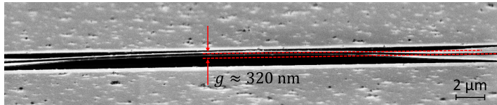
(b) Partially released reference waveguide.
