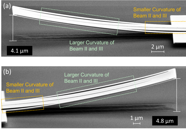
Figure 6.14: SEM images of two four-beam structures of pure Si after Step (c) of the fabrication process. Structural dimensions are: (a) l_{\text{SMA}} = 30 \mu\text{m} , w_{\text{SMA}} = 2.2 \mu\text{m} , l_{\text{Si}} = 25 \mu\text{m} , w_{\text{Si}} = 1.0 \mu\text{m} ; (b) l_{\text{SMA}} = 40 \mu\text{m} , w_{\text{SMA}} = 2.7 \mu\text{m} , l_{\text{Si}} = 25 \mu\text{m} , w_{\text{Si}} = 0.7 \mu\text{m} . The dashed frames indicate the regions with curvatures difference between Beam I and Beam II. The deflections at the free-ends of the beams are marked out in the pictures.
