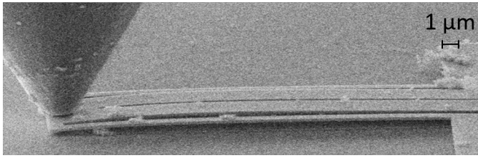
(b) Buckled up state
