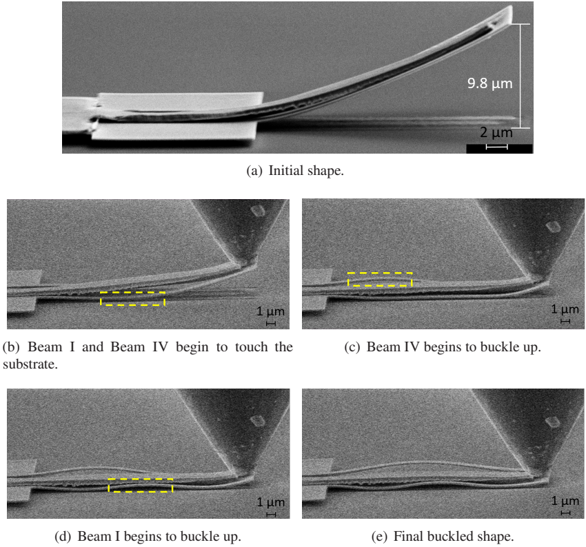
Figure 6.21: SEM images show the deformed structural shapes during the loading process. The corresponding moments (a)–(e) are marked in Fig. 6.20.
