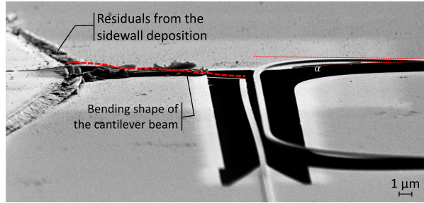
(b) Side view of Structure B.
