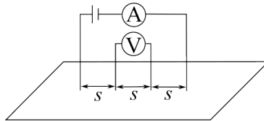
Figure 2.3: Sketch of the four-point measurement setup for thin film samples.
