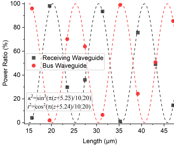
Figure 7.24: The ratios of power outputs from the receiving and the bus waveguides of different lengths at the wavelength of 1550 nm. The dots are experimental data, and the dashed lines are curves of the fitted functions.
