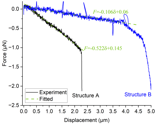
Figure 6.18: Relations between the displacement and the reaction force (solid lines) recorded by the nanoindenter, which can be fitted by linear functions (dashed lines). Dimensions of the tested structures are: l_{\text{SMA}} = 20 \mu\text{m} , w_{\text{SMA}} = 2.2 \mu\text{m} , l_{\text{Si}} = 15 \mu\text{m} , w_{\text{Si}} = 0.7 \mu\text{m} for Structure A; l_{\text{SMA}} = 30 \mu\text{m} , w_{\text{SMA}} = 2.2 \mu\text{m} , l_{\text{Si}} = 25 \mu\text{m} , w_{\text{Si}} = 0.7 \mu\text{m} for Structure B.
