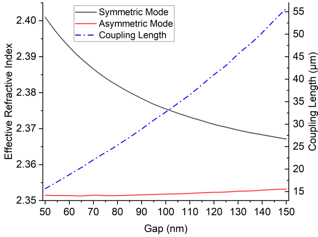
Figure 7.6: Influence of gap size of the directional coupler on symmetric and asymmetric effective refractive indices and the coupling length simulated at the wavelength \lambda of 1550 nm.
