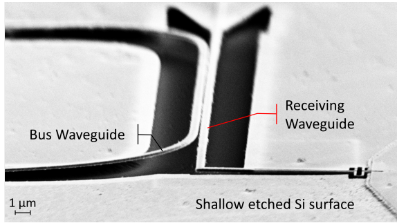
(a) Free-standing directional coupler with a cantilever beam.
